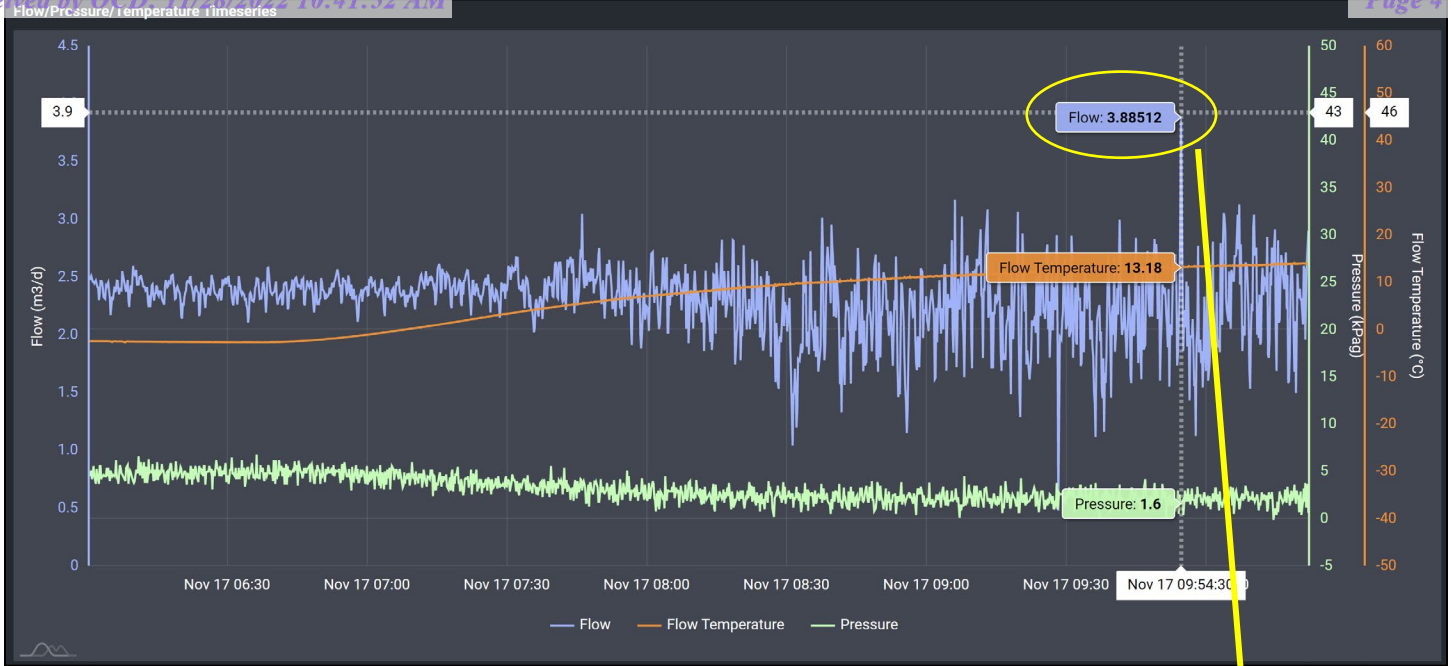
Image 4.1 – Double L Queen #03Q (30-005-20338) Methane Flow/Pressure/Temperature Timeseries & Peak Flow at Interval #1 testing period of 4.4-hours.
