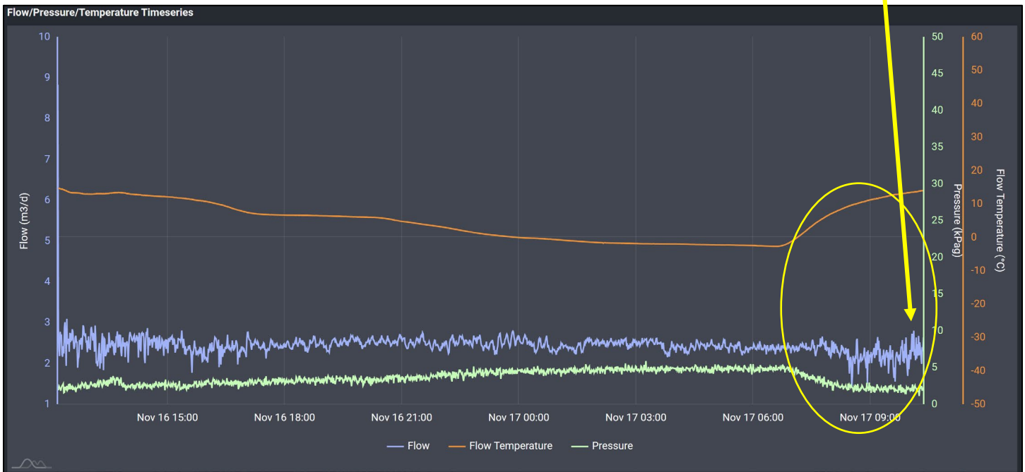
Image 4.2 – Double L Queen #03Q (30-005-20338) Methane Flow/Pressure/Temperature Timeseries & Peak Flow for entire testing period of 22.2-hours.
