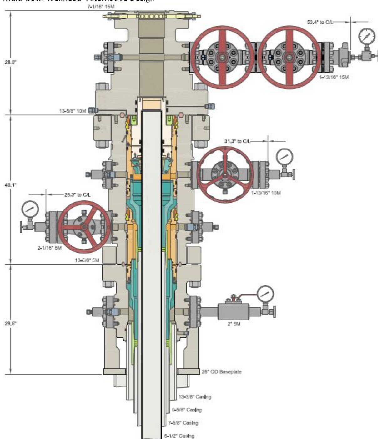
Multi-bowl Wellhead- Alternative Design
