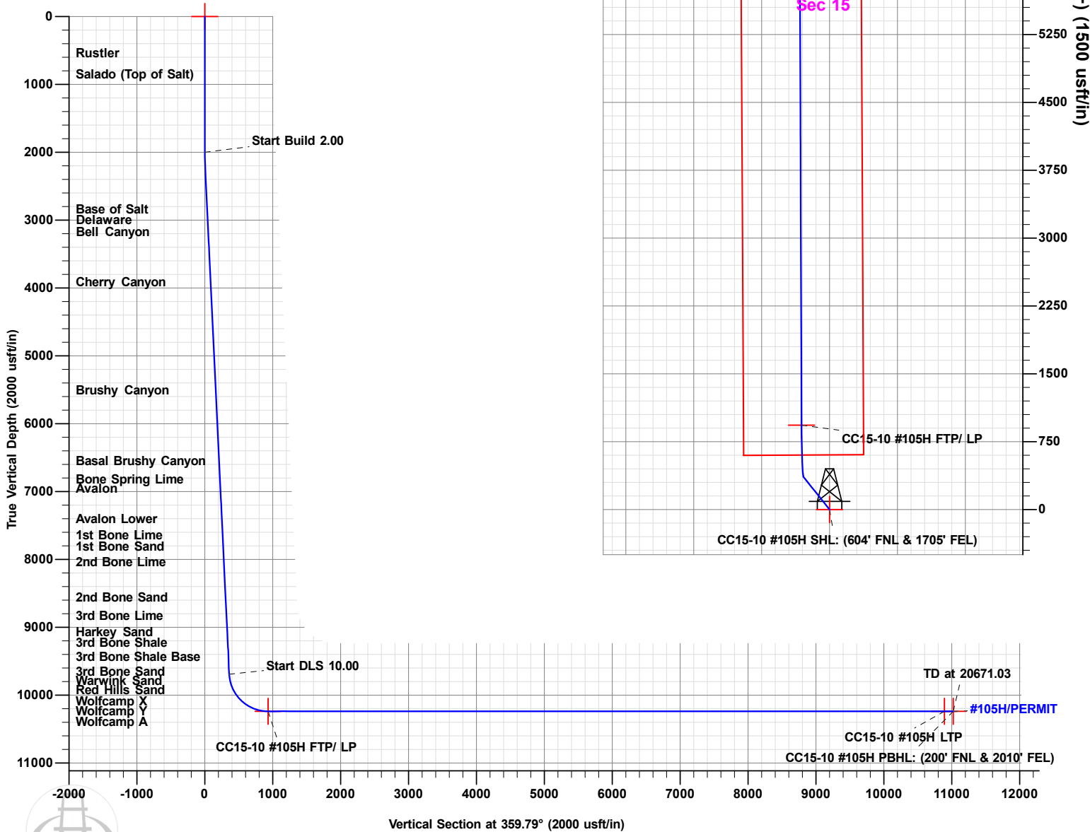
Vertical Section at 359.79° (2000 usft/in)
