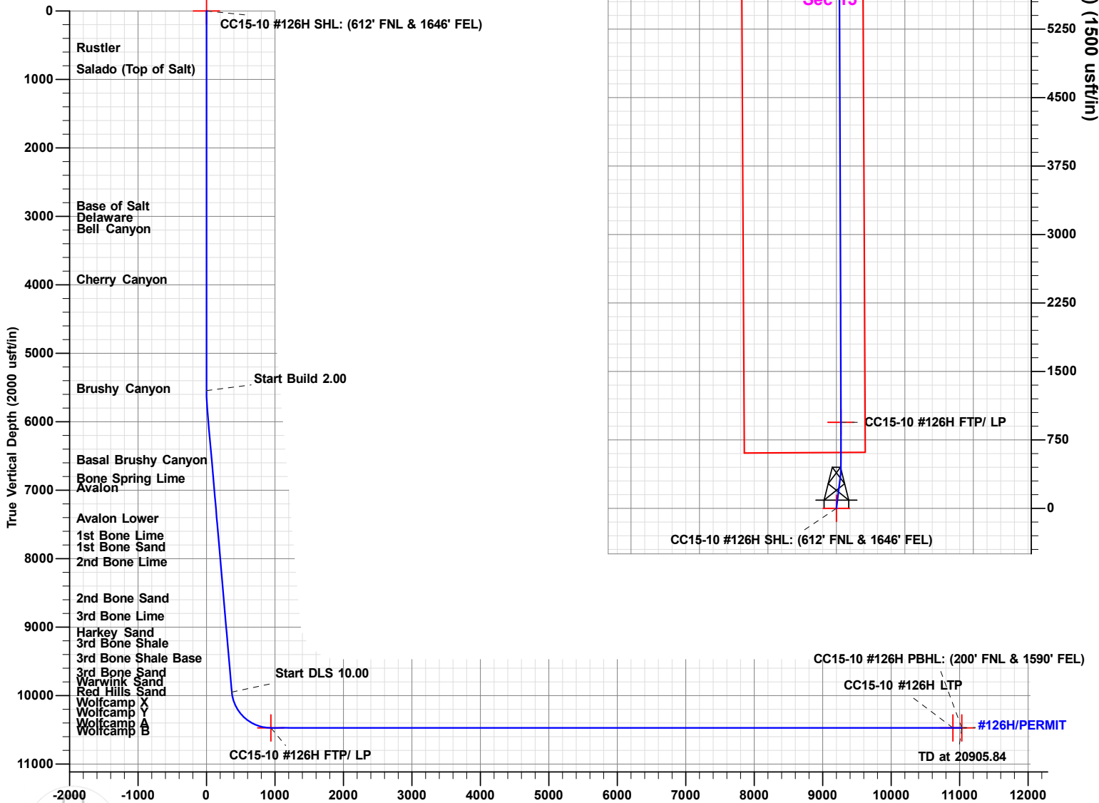
Vertical Section at 359.79° (2000 usft/in)
