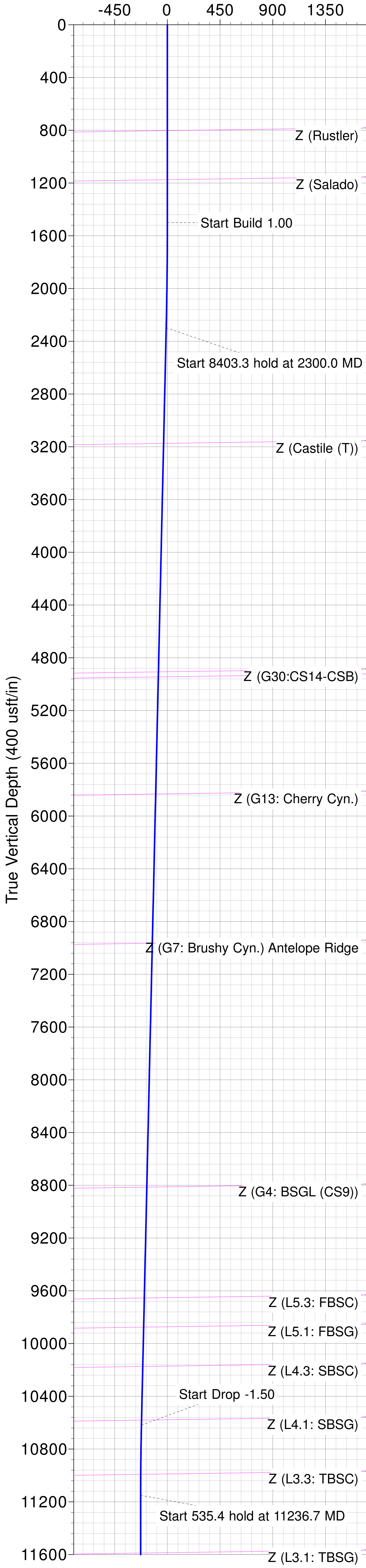
Vertical Section at 359.61° (450 usft/in)
