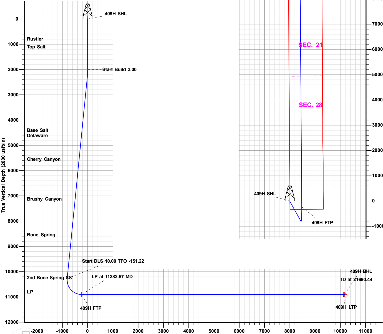
Vertical Section at 359.59° (2000 usft/in)
