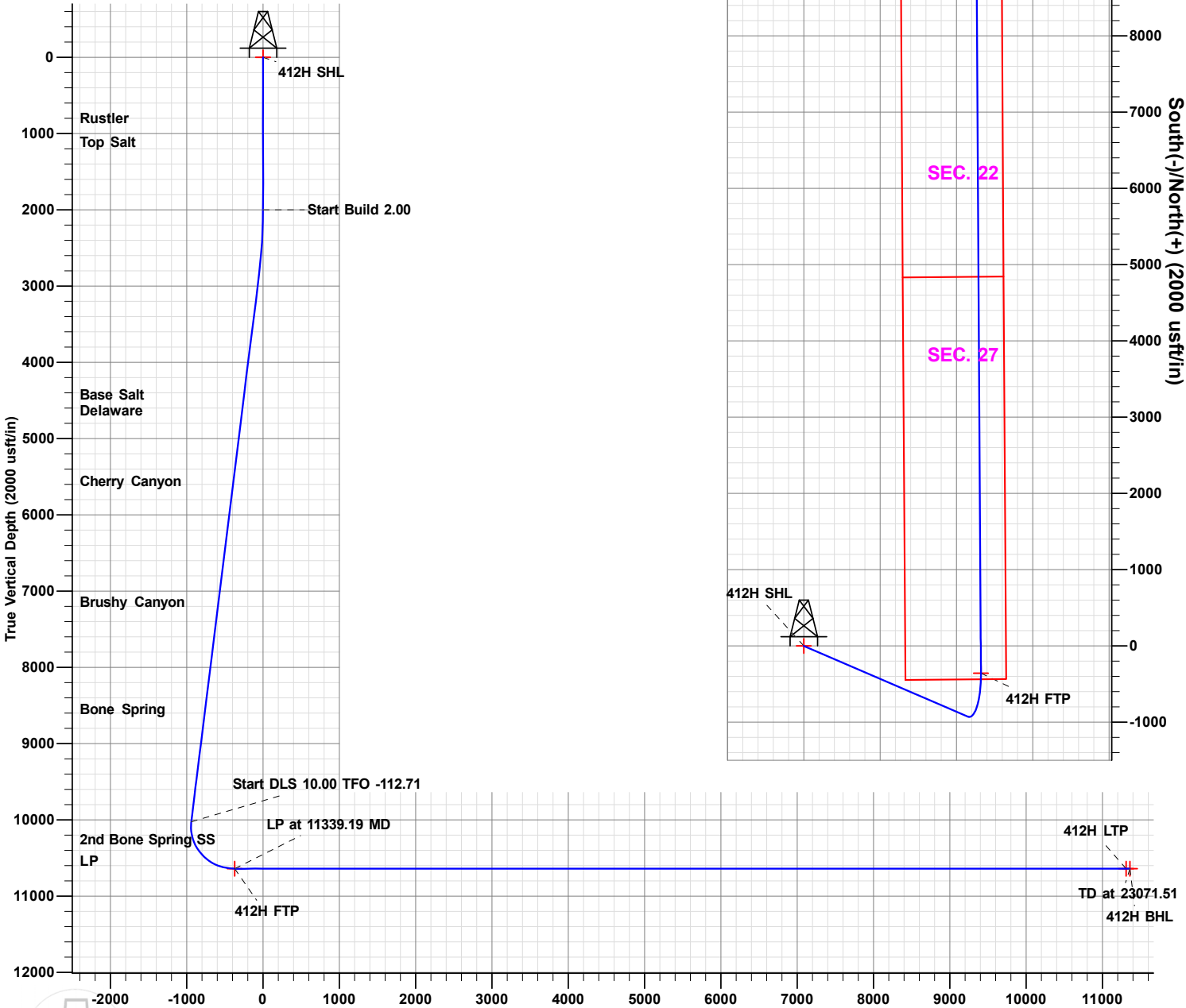
Vertical Section at 359.65° (2000 usft/in)
