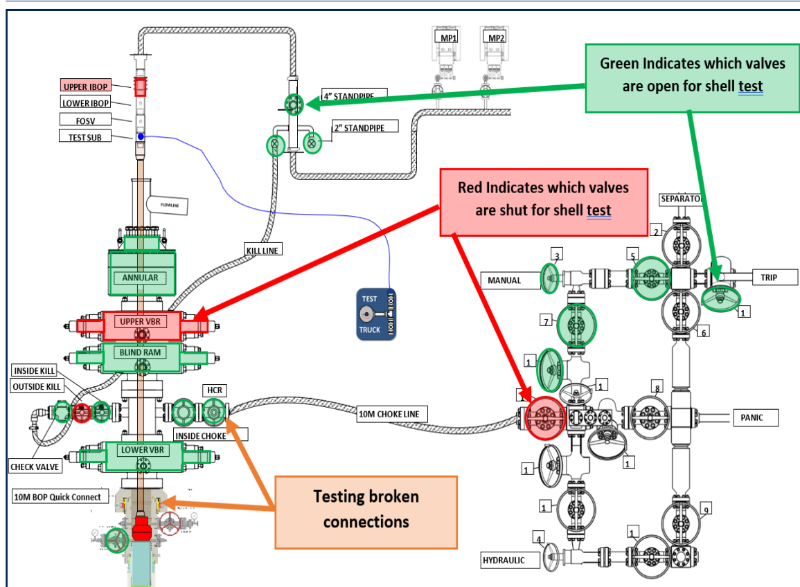
Figure 4: Shows which valves are shut/open for the shell test, testing both broken connections
