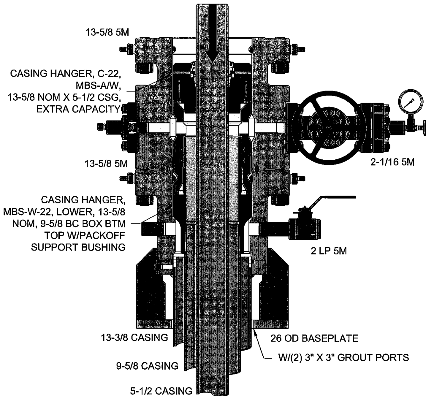
FIGURE 4 – HANGER INSTALLED
