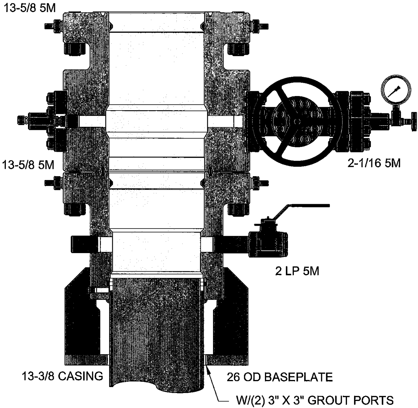
FIGURE 1 – LANDING MULTI-BOWL
