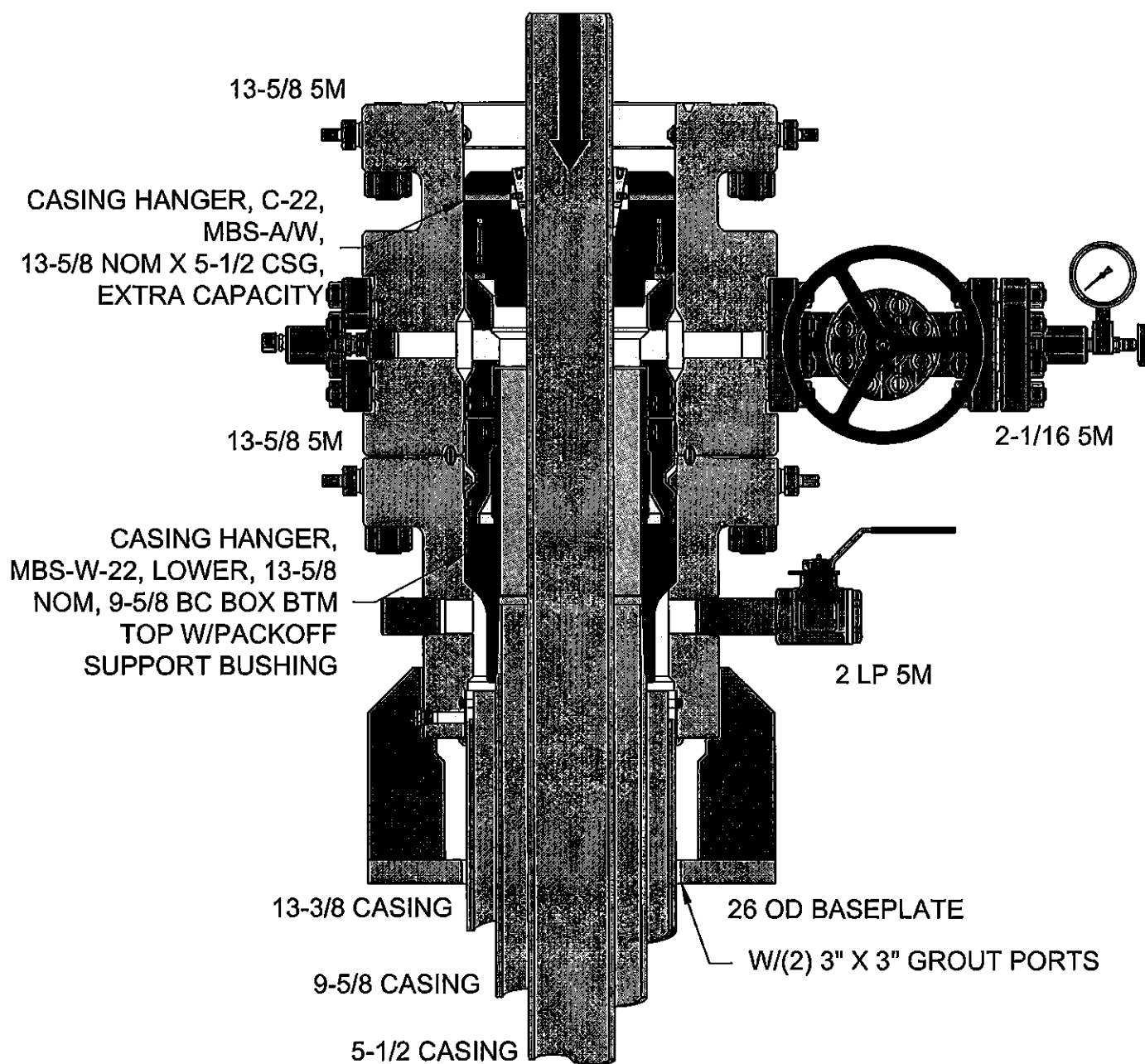
FIGURE 4 – HANGER INSTALLED
