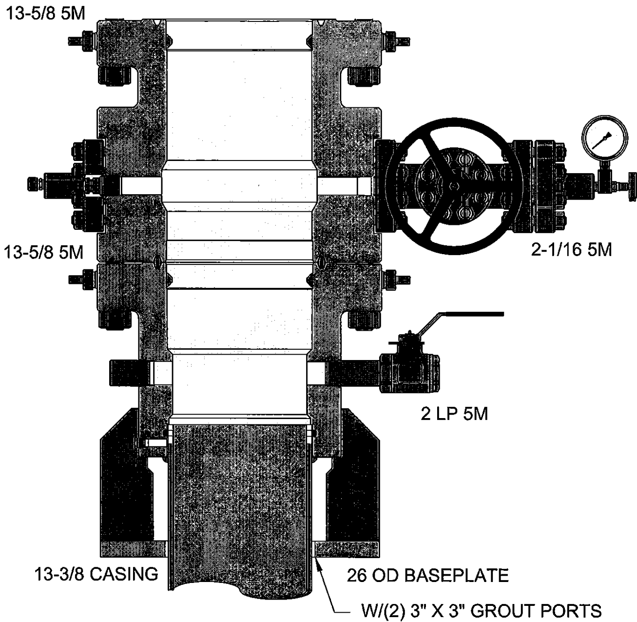
FIGURE 1 – LANDING MULTI-BOWL
