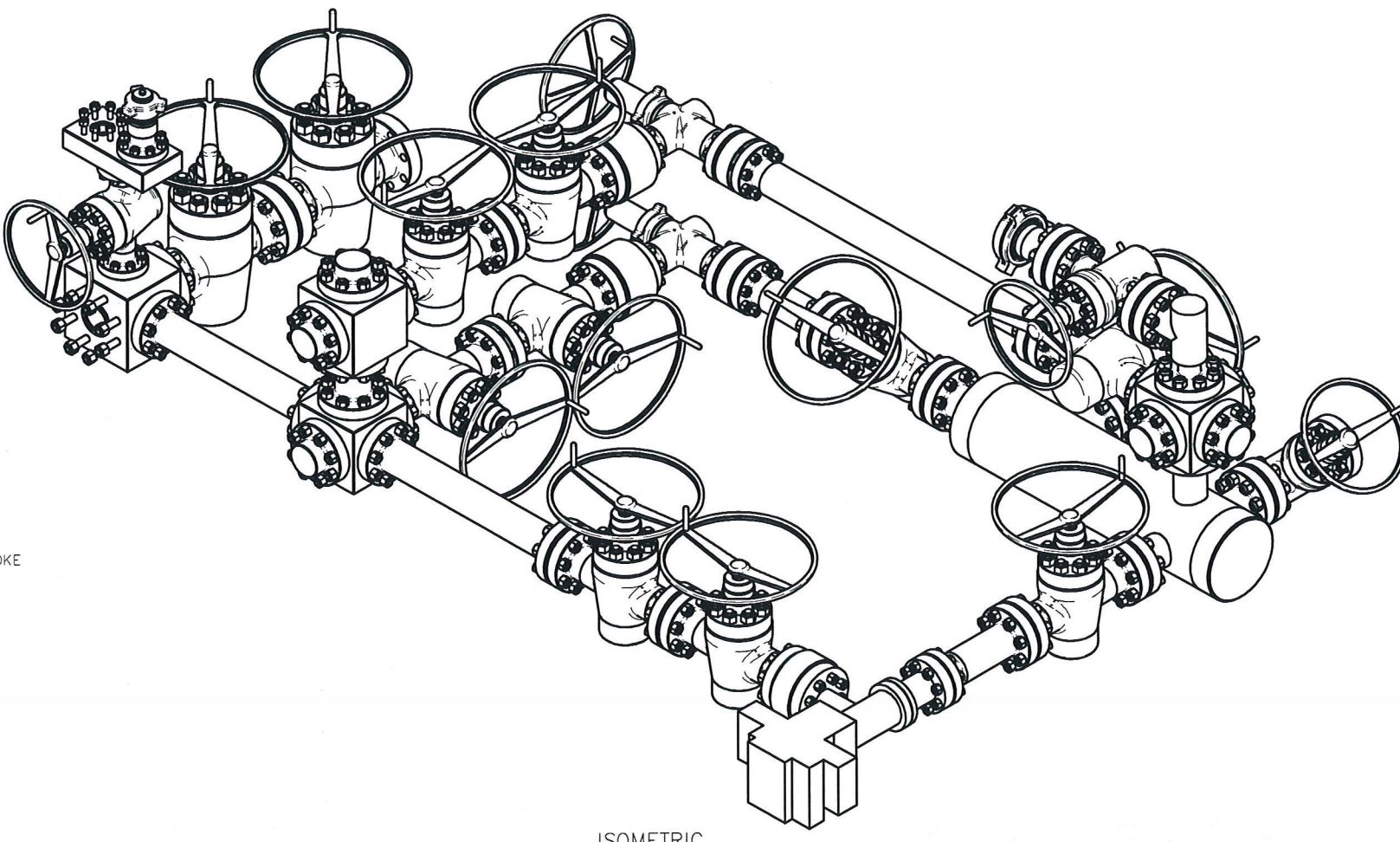
ISOMETRIC
