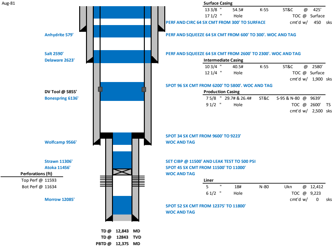
Proposed Wellbore
