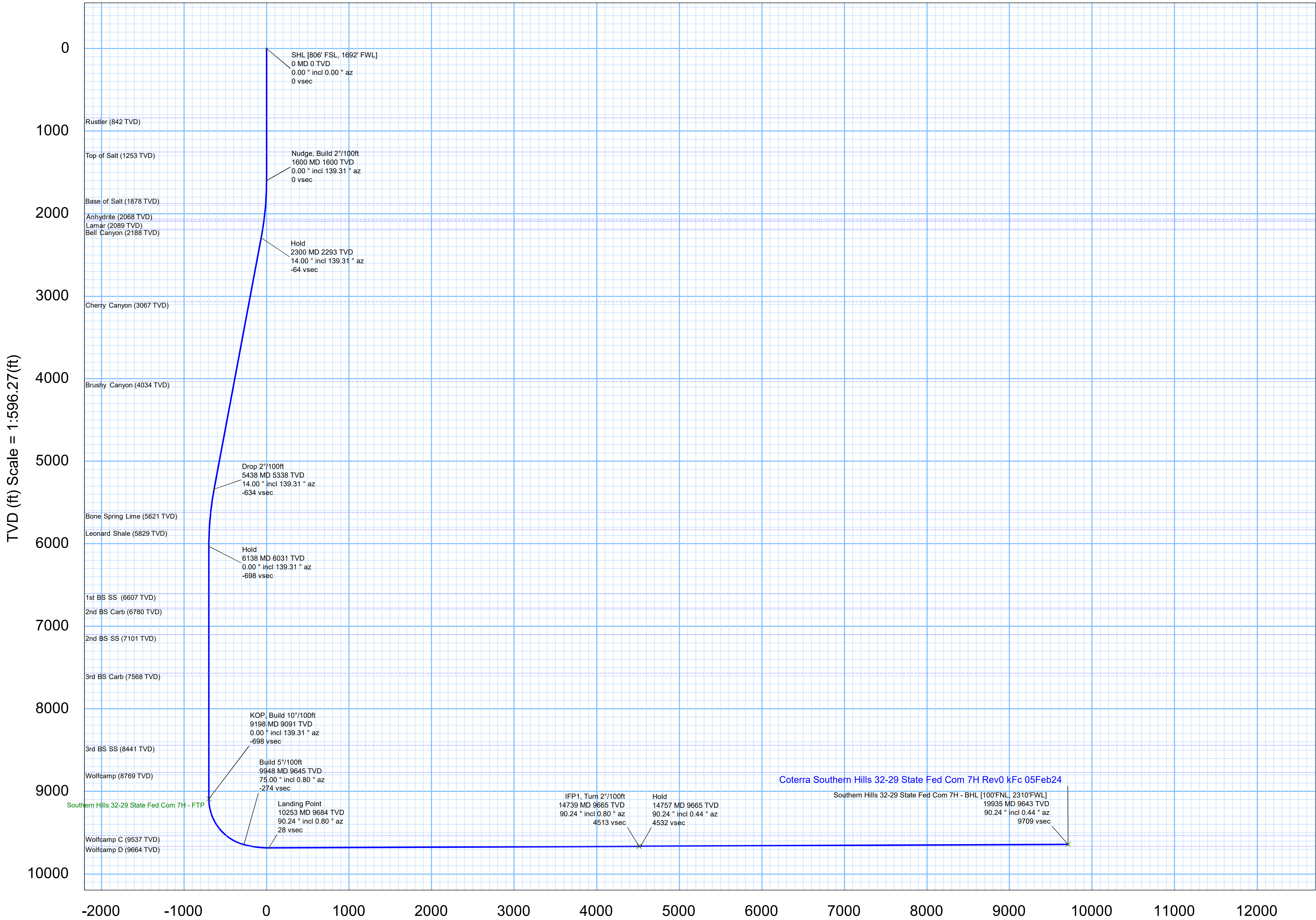
Vertical Section (ft) Azim = 0.62° Scale = 1:596.27(ft) Origin = 0N/-S, 0E/-W
