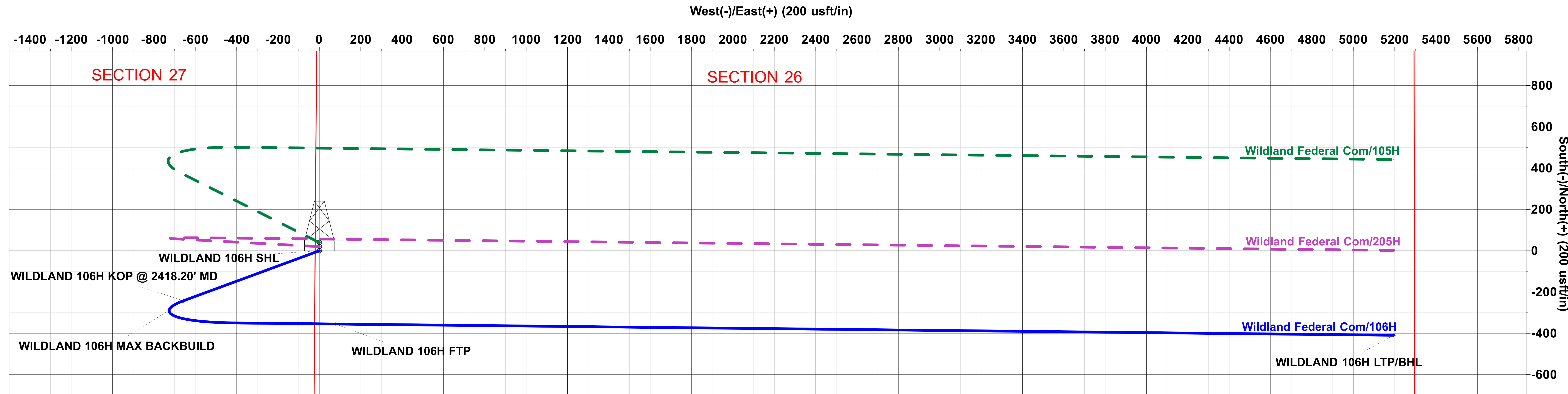
WELL DETAILS: 106H
