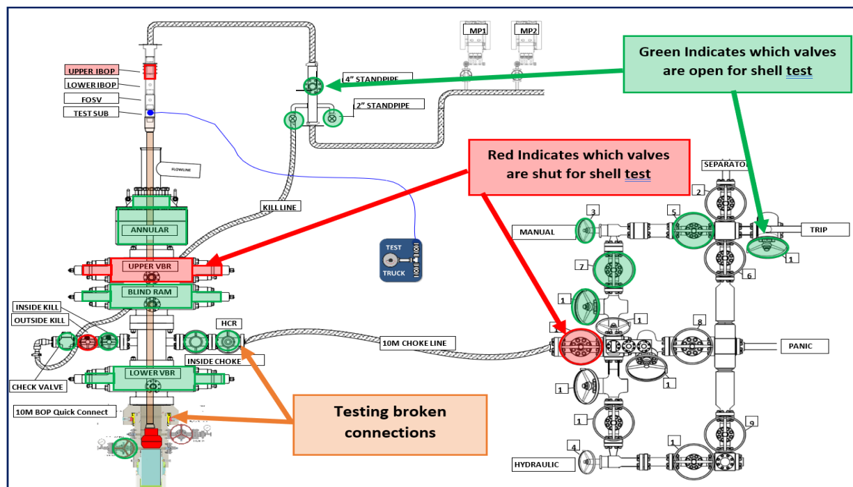
Figure 4: Shows which valves are shut/open for the shell test, testing both broken connections
