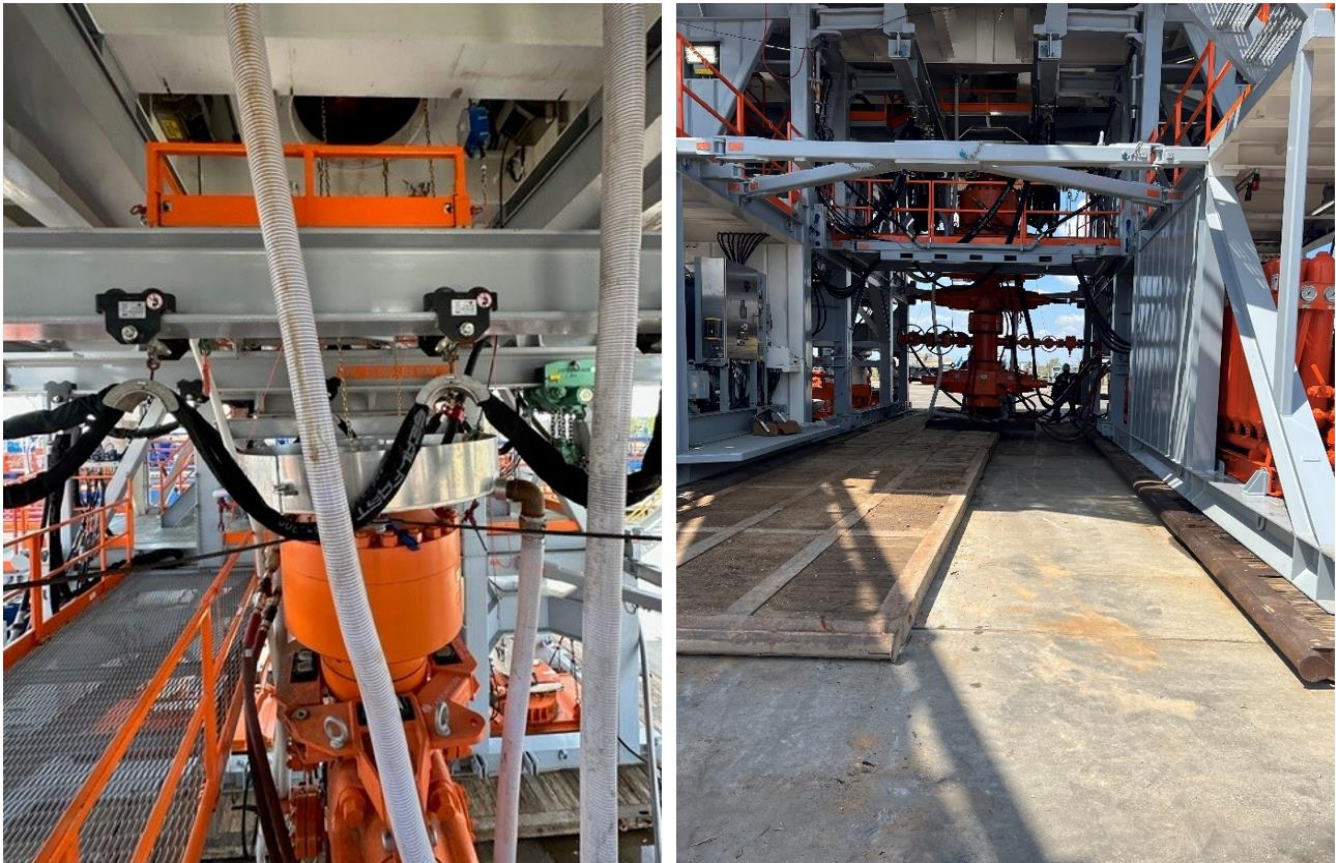
Figures 1 & 2: BOP winch system picture with walking capabilities.
