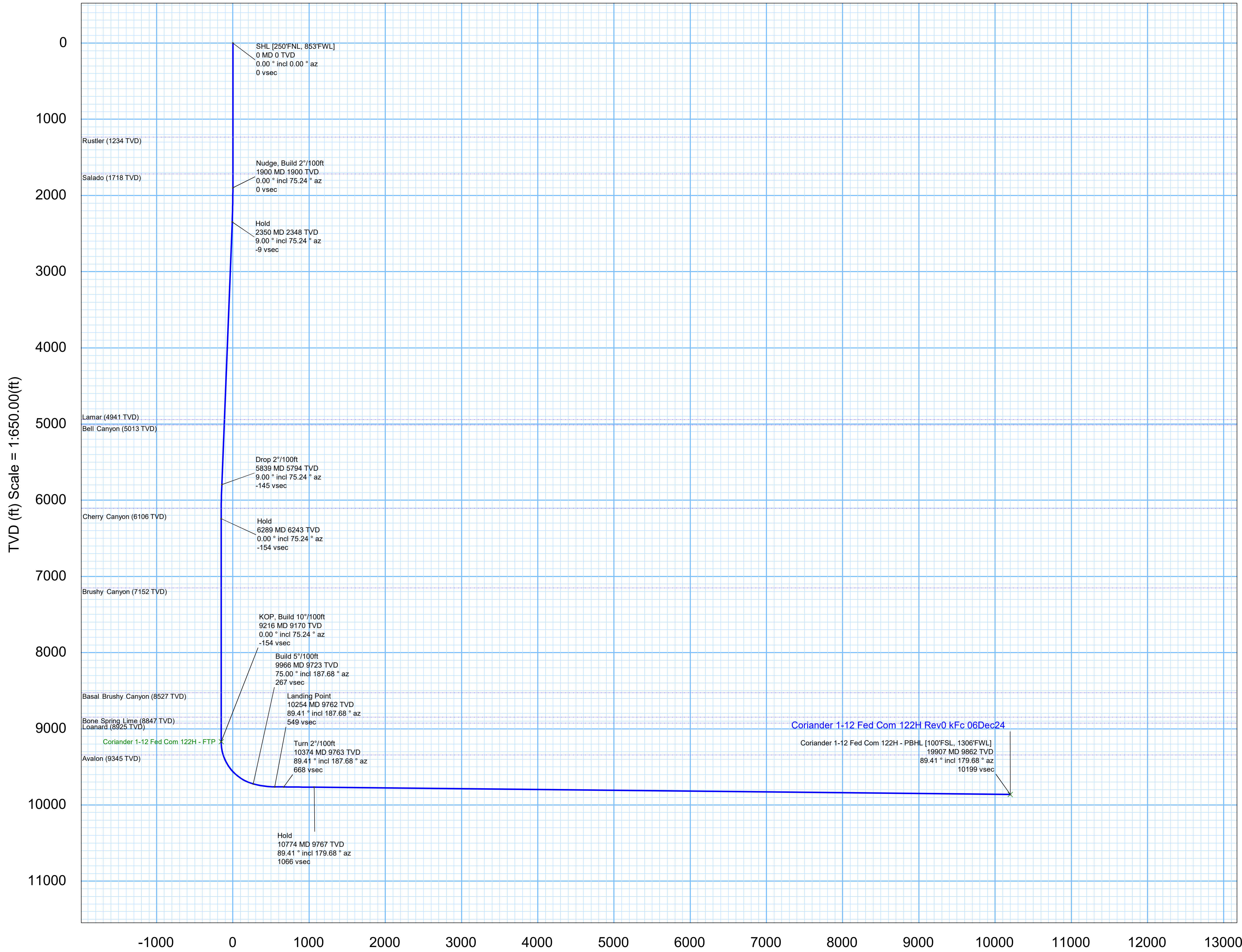
Vertical Section (ft) Azim = 179.68° Scale = 1:650.00(ft) Origin = 0N/-S, 0E/-W
