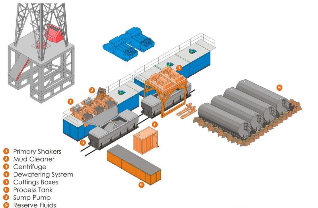
Closed Loop Schematic
