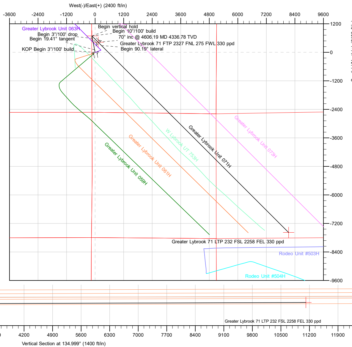
Vertical Section at 134.999° (1400 ft/in)
