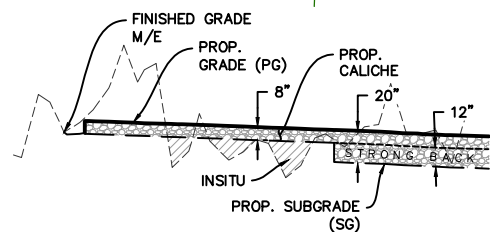
TYPICAL SECTION DETAIL NOT TO SCALE
