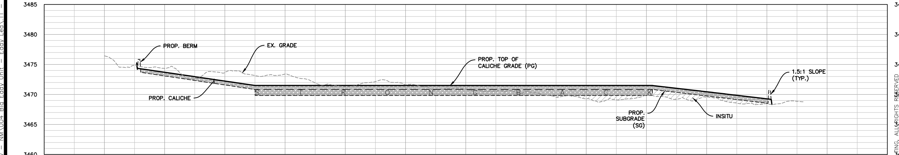
CROSS SECTION "B" H: 1" = 200' V: 1" = 20'
