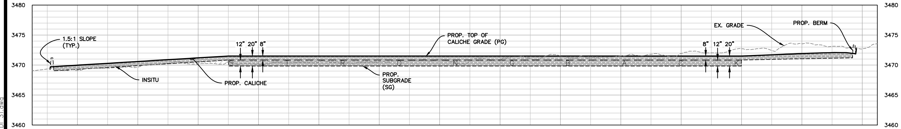
CROSS SECTION "E" H: 1" = 200' V: 1" = 20'
