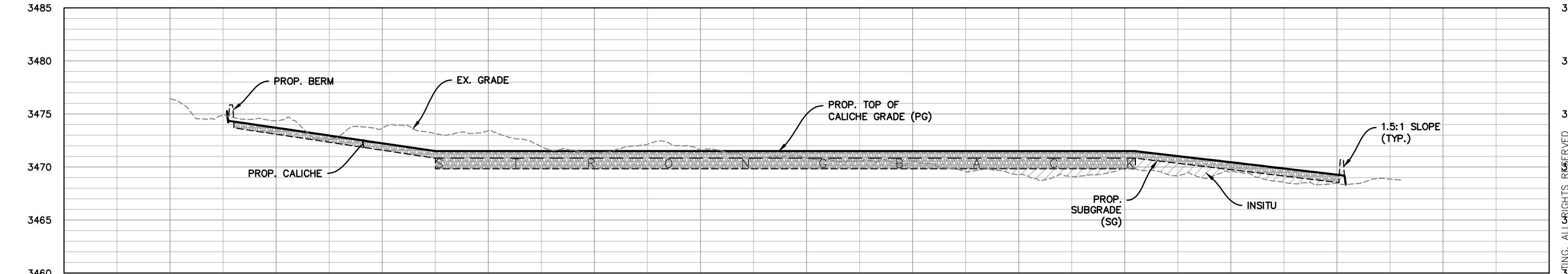
CROSS SECTION "B" H: 1" = 200' V: 1" = 20'
