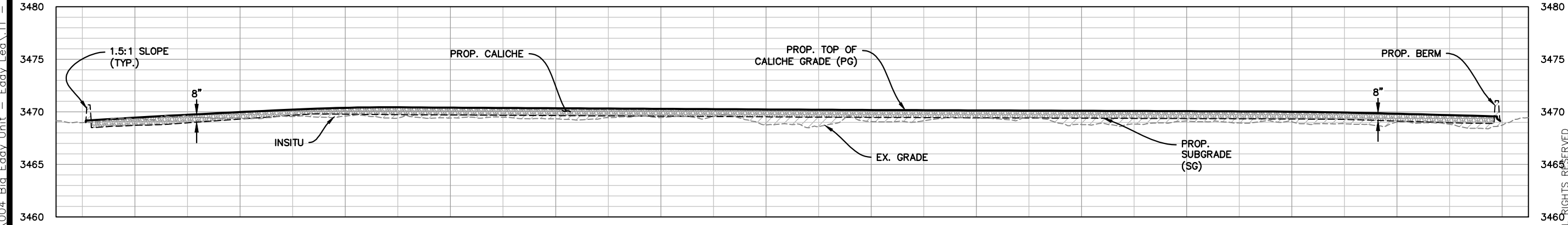
CROSS SECTION "F" H: 1" = 200' V: 1" = 20'
