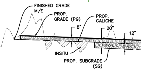
TYPICAL SECTION DETAIL NOT TO SCALE
