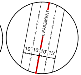
TYPICAL N.T.S. RIGHT-OF-WAY EASEMENT, CONFIGURATION (L10)
