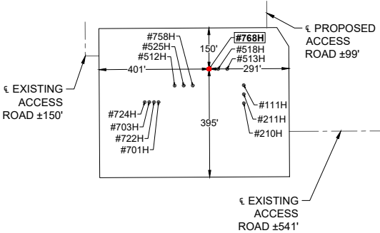
DETAIL VIEW SCALE: 1" = 500'
