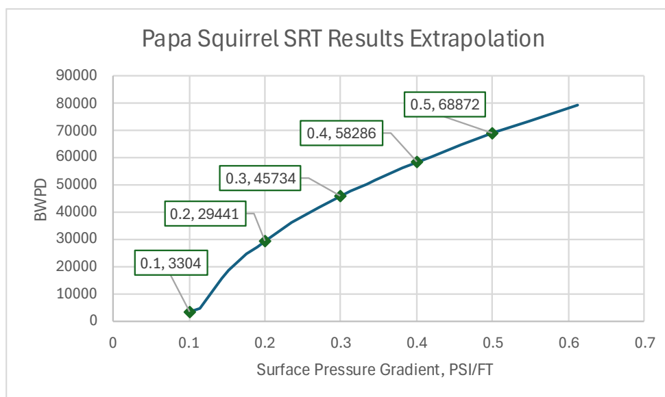
Figure 5: Extrapolating Papa Squirrel’s SRT results illustrates the well’s injection potential with different surface injection pressure gradients.
