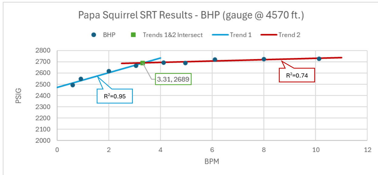
Figure 3: Plot of Composite Bell & Cherry Canyon Step Rate Test Data – Injection Rate vs Downhole Gauge. Fracturing conditions at intersection of trend lines are 3.31 bpm and 2689 psig at the downhole gauge depth of 4570 ft. Using 9.1 ppg brine and assuming negligible friction this is ~2729 psig at the top of the permitted interval at 4654 ft or ~2733 psig at the top perf at 4662 ft.
