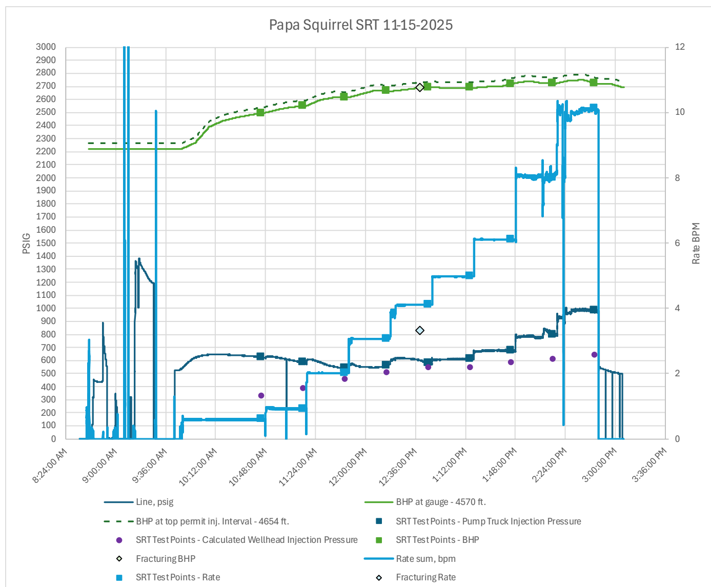
Figure 4: Plot of Step Rate Test Data vs Time including Injection Rate, Pump Truck Injection Pressure, Downhole Gauge Pressure, Calculated Pressure at the top of the permitted injection interval, Calculated Wellhead Injection Pressure, Points Taken for SRT analysis, and Fracturing Rate/Pressure. The plot illustrates discrepancy between measured pump truck injection pressures and calculated wellhead injection pressure given known fluid density and BHP measurements.
