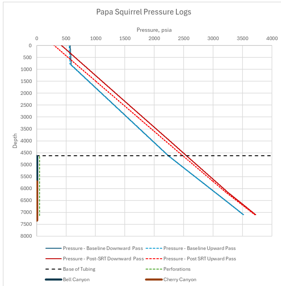
Figure 1: Pressure logs pre and post SRT.
