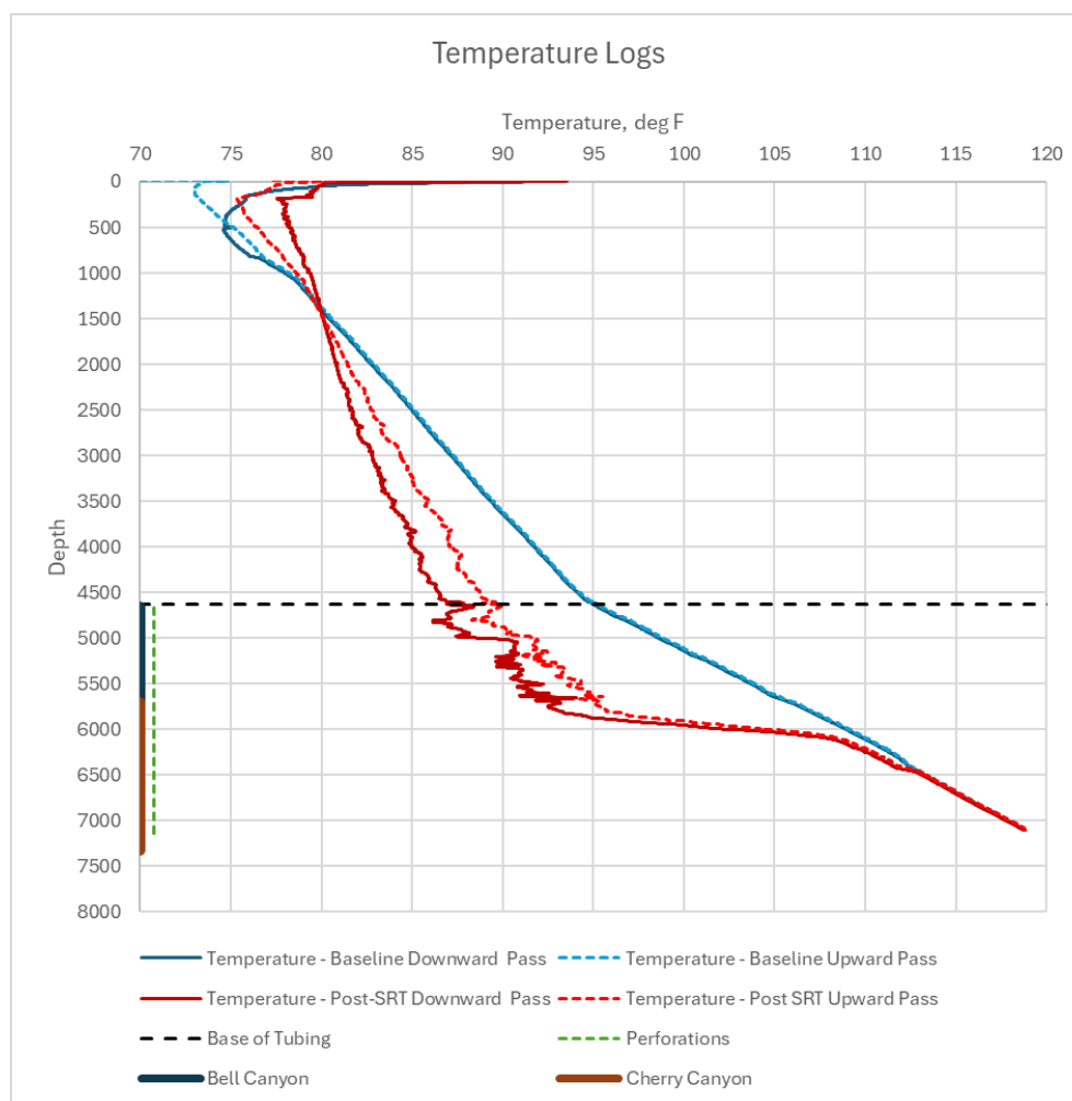
Figure 2: Temperature logs pre and post SRT.
