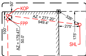
DETAIL VIEW SCALE: 1" = 600'
