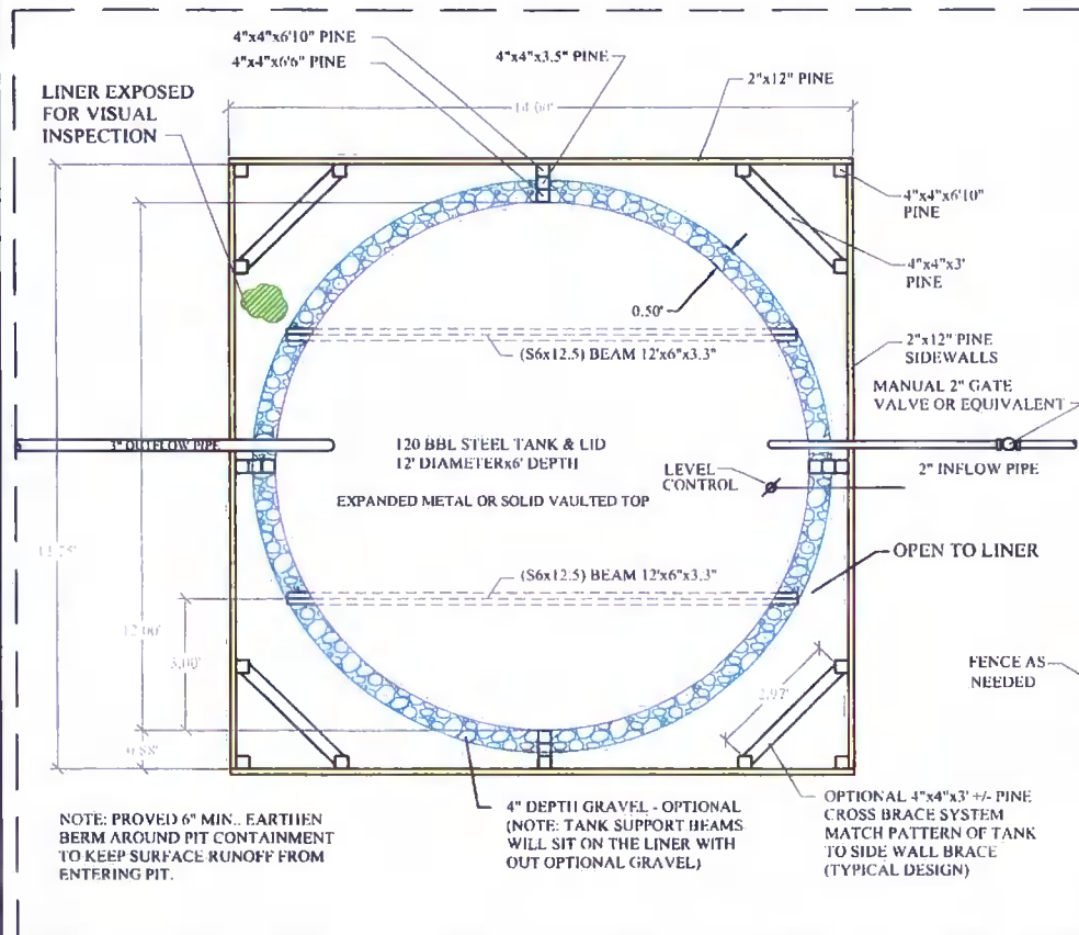
PLAN VIEW
