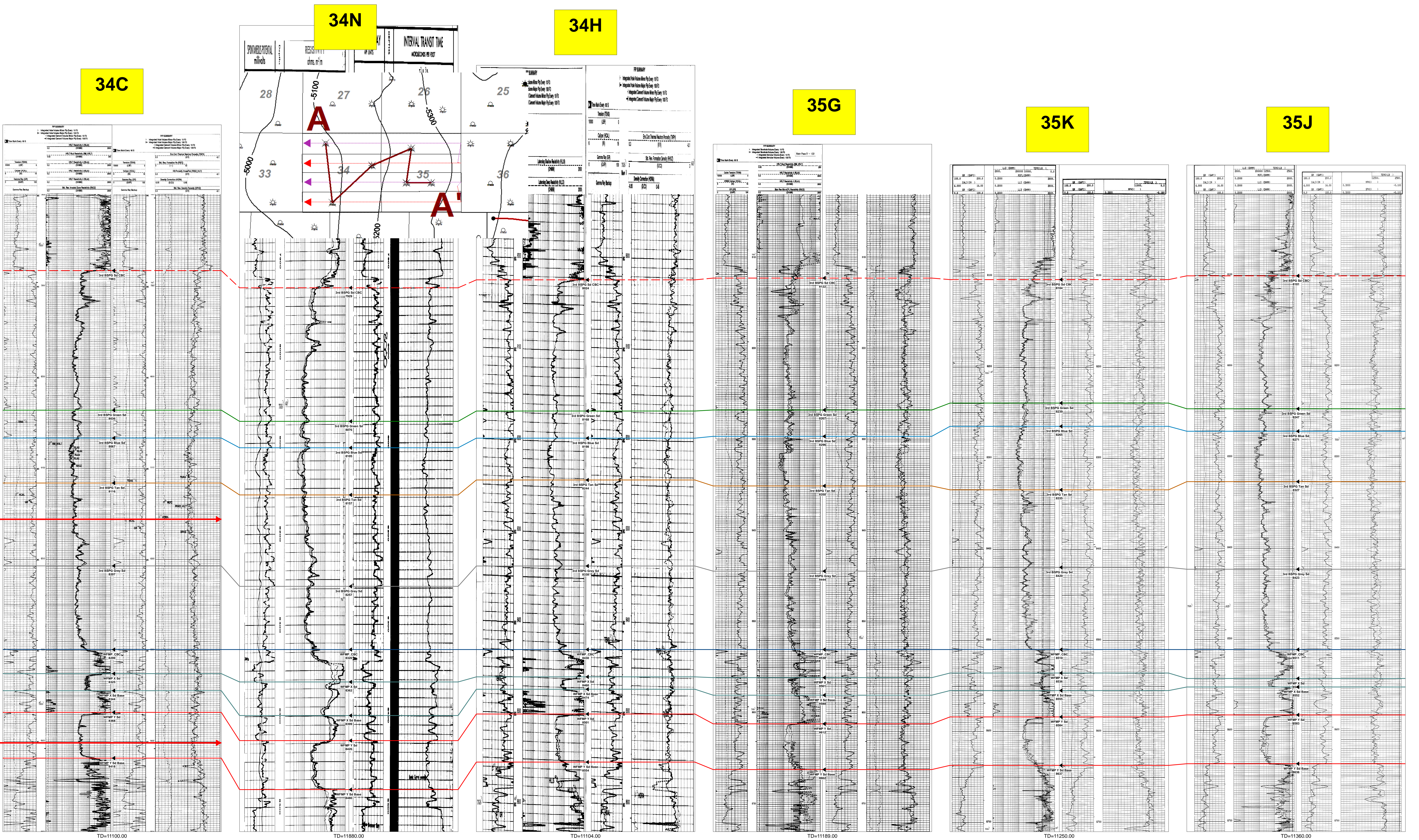
Cripple Creek 35/34 3rd BSPG SD-WFMP SD Cross Section Exhibit (A-A')
