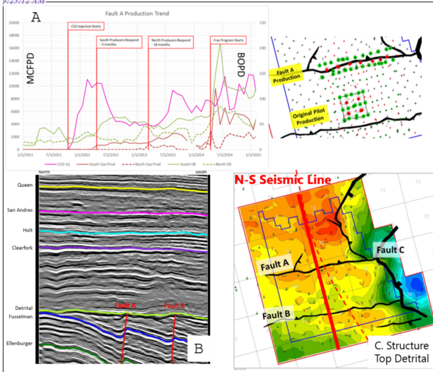
A. Fault "A" Production Trend showing delayed response of wells north of deep-seated fault and shallow fractures. B North-South Seismic Line. C. Top Pennsylvania Detrital structure map with north-south seismic line.
