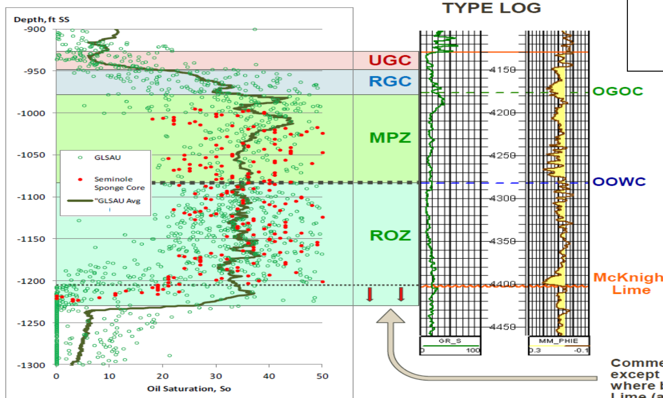
Core Oil Saturations Resaturated Gas Cap, Main Pay, and ROZ for Goldsmith Landreth San Andres Unit, Goldsmith Field, Ector County, TX.
