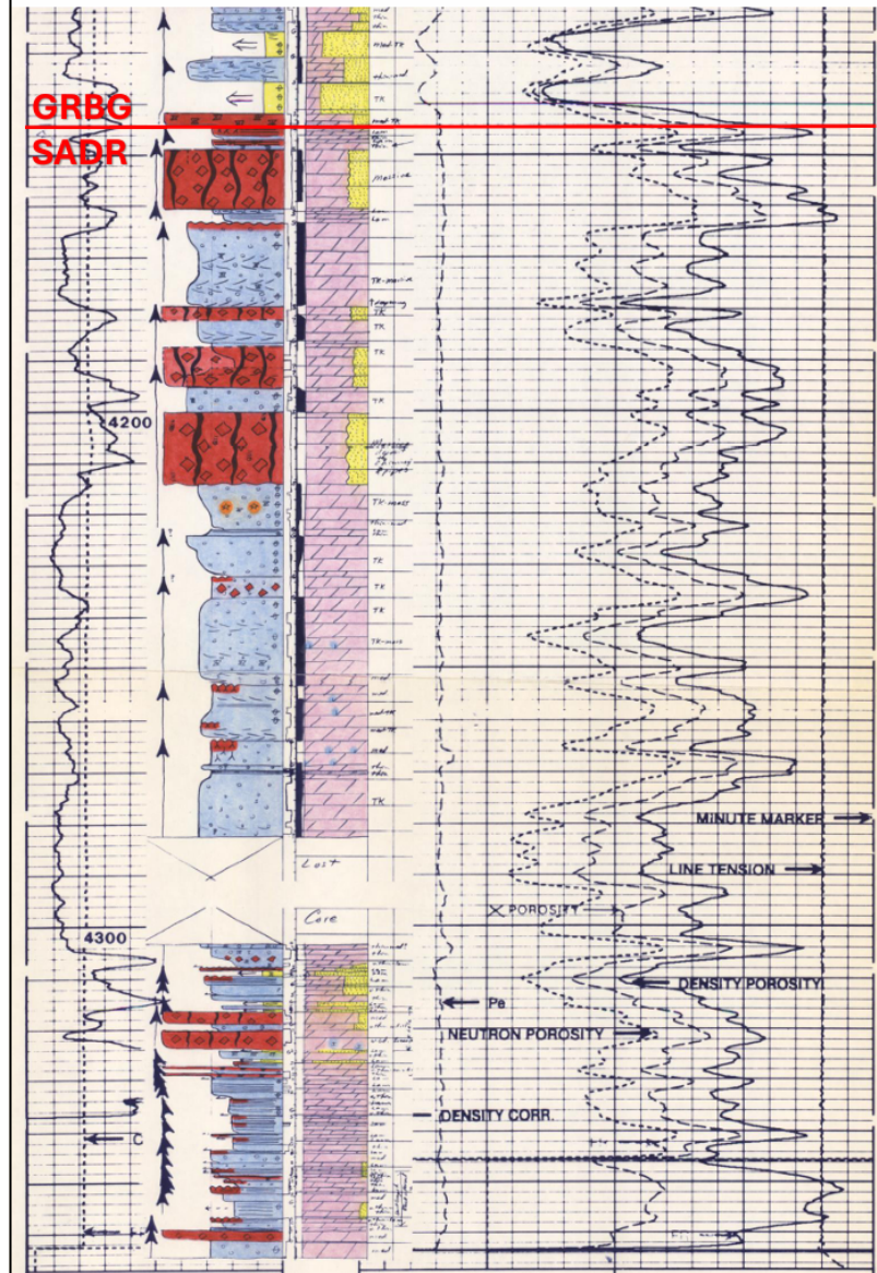
EMSU-679 basal Grayburg and upper San Andres well log, core description, and core photographs (Plain light and UV) showing porous oil-stained strata.
