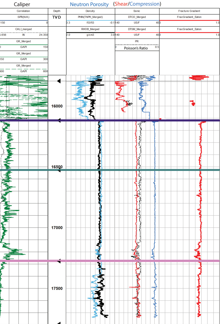
Figure 10. Fracture pressure gradient empirically derived for Independence AGI #1 (red trace). Average fracture gradient estimates range from 0.667 to 0.693 psi/ft. for Devonian through Fusselman geologic strata.
