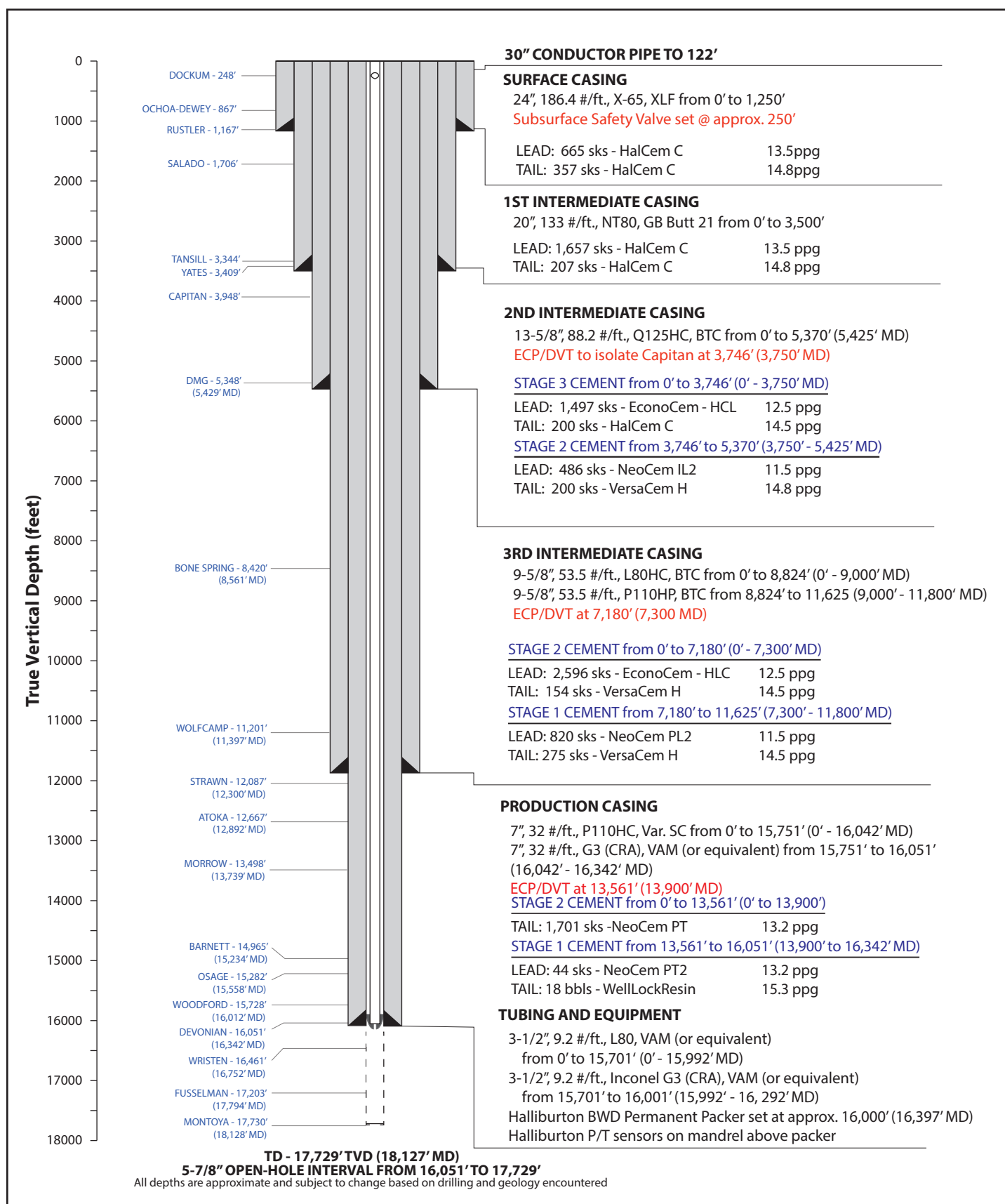
Figure 4. Proposed Independence AGI #3 well schematic.
