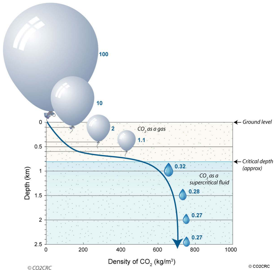
Figure A-26: Density of Carbon Dioxide as a Function of Depth.
