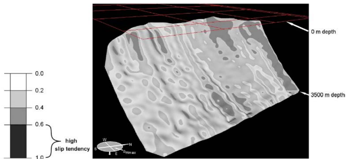
Figure A-13: Example Fault Slip Tendency Image.
