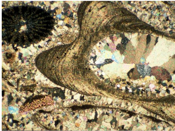
Figure A-5: Limestone With Fossil Fragments, Viewed under Crossed Polarizers.
