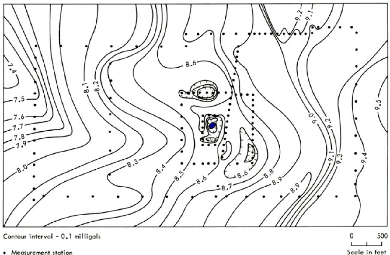
Figure A-18: A Gravity Map of an Area Ore Deposit and Mine.
