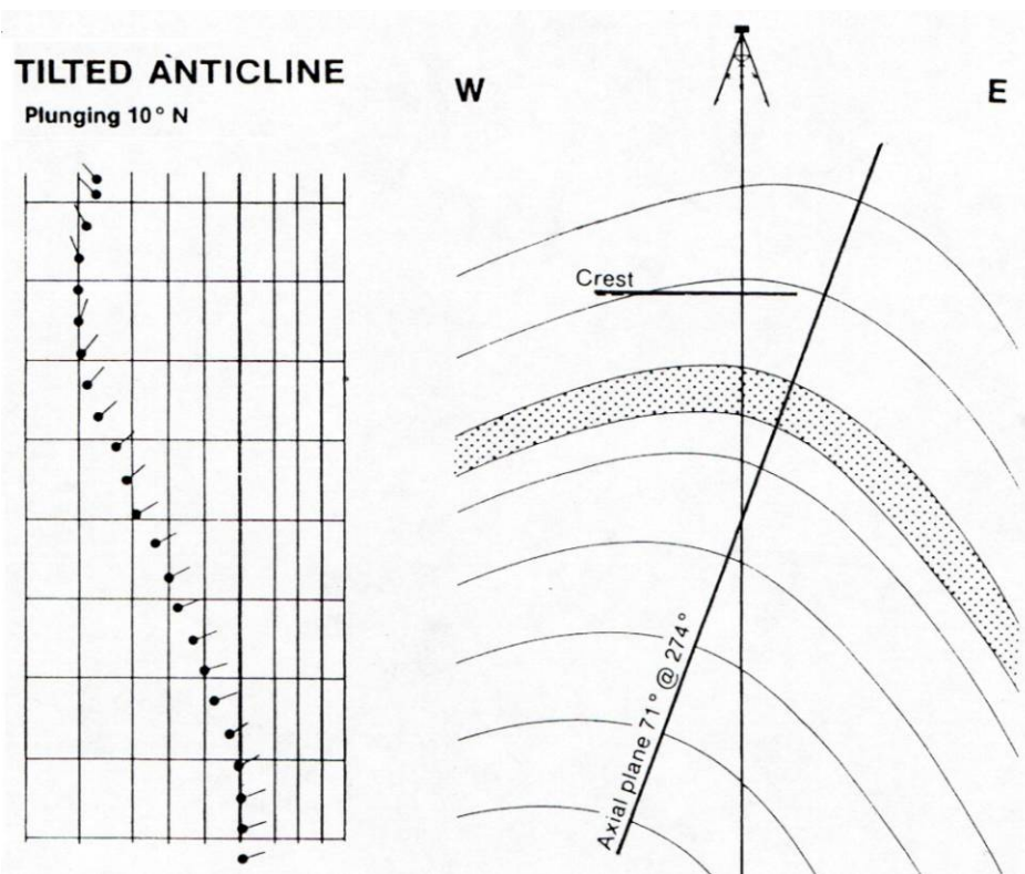
Figure A-3: Dip Model of a Tilted Plunging Anticline as it would Appear on an Arrow Plot of Dipmeter.
