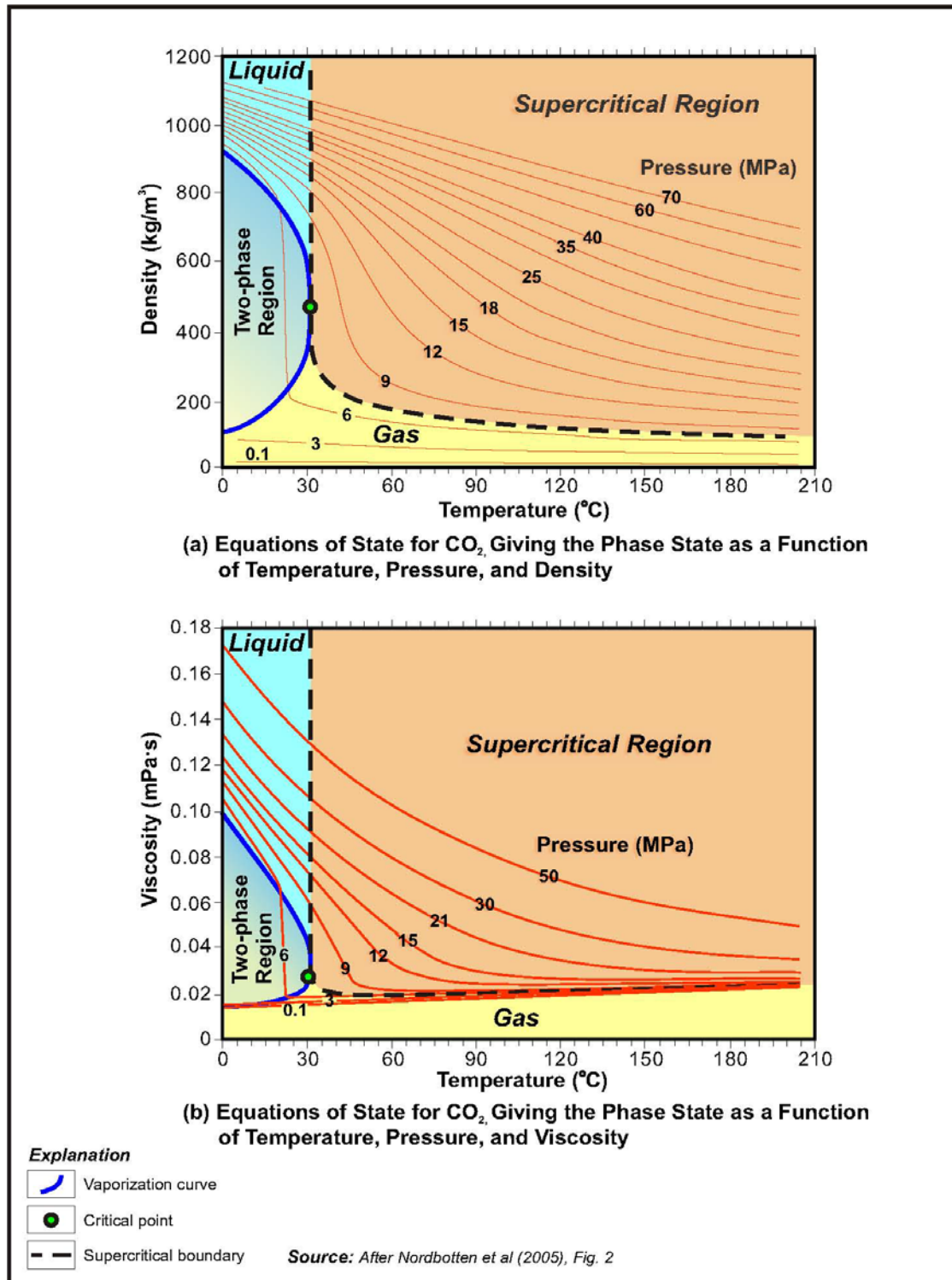
Figure 2-1: Equations of State for Carbon Dioxide.
