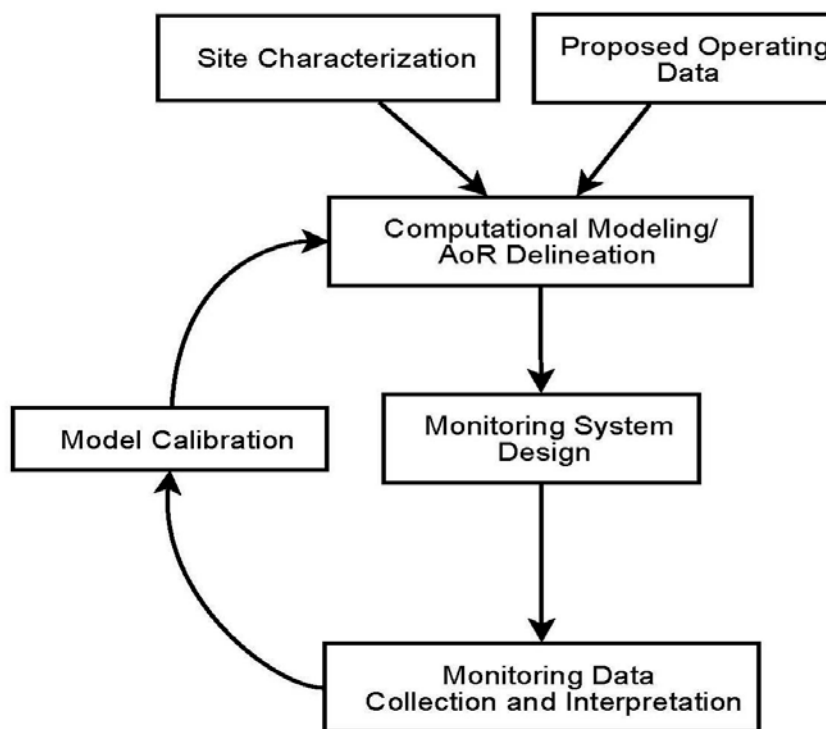
Figure 4-1. Flow chart of modeling and monitoring at a Class VI project.
