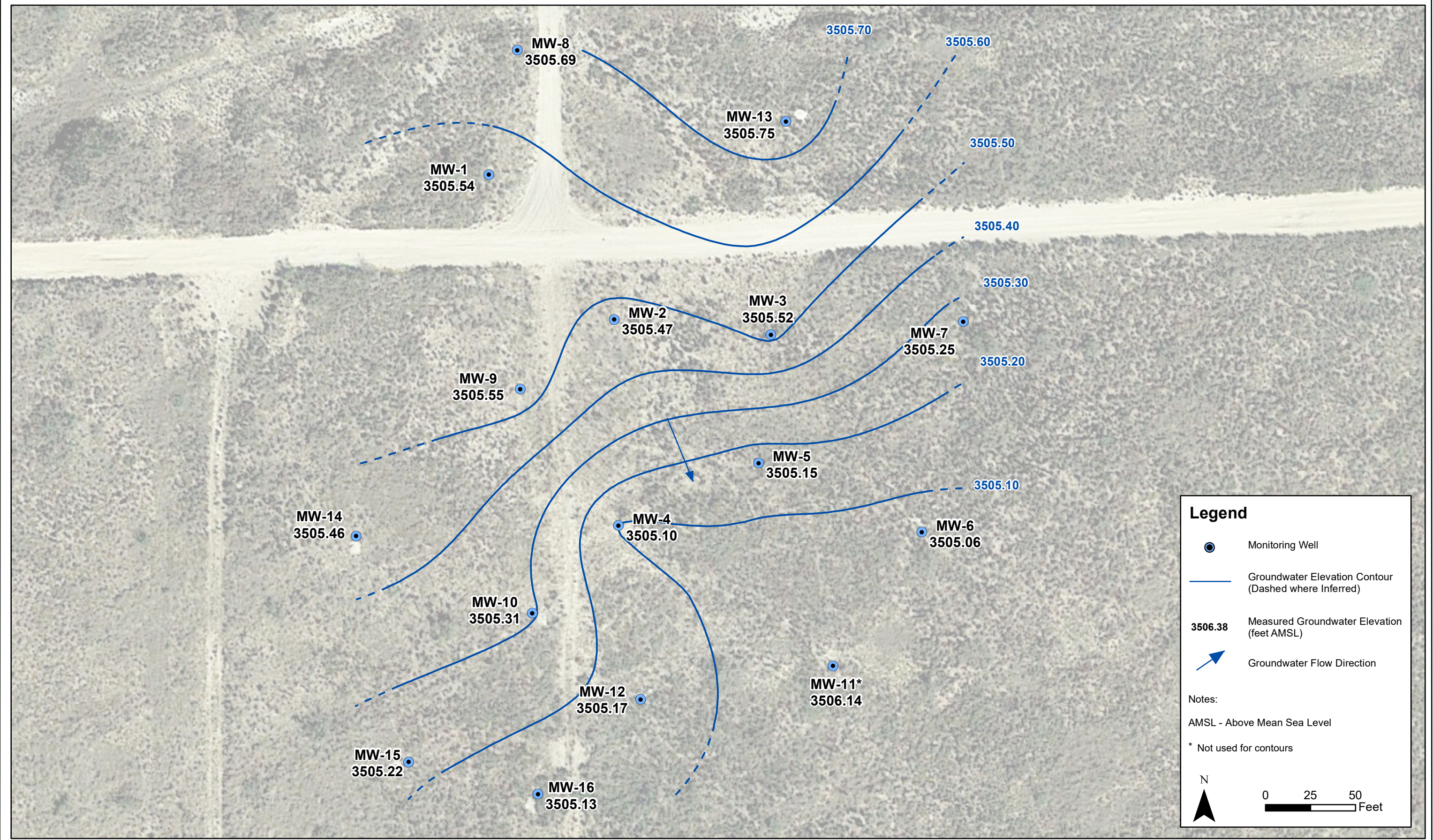
Groundwater Elevation Contour Map (December 20, 2021)
