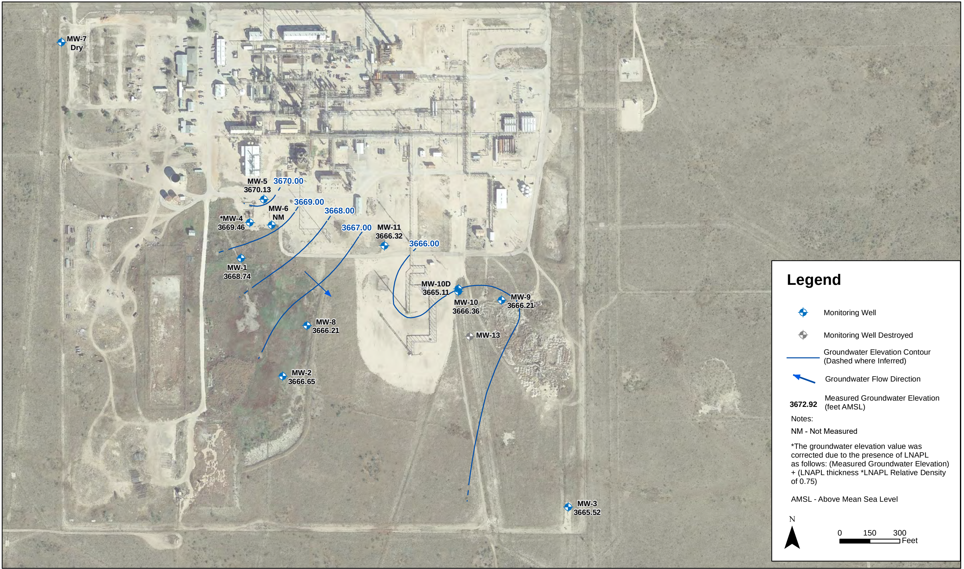
Groundwater Elevation Contour Map (March 25, 2021)
