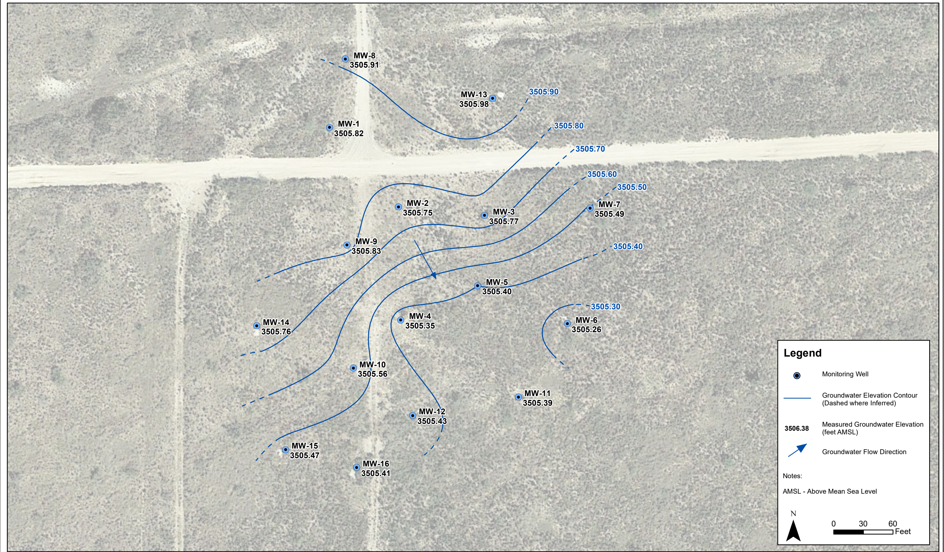
Groundwater Elevation Contour Map (December 14, 2020)
