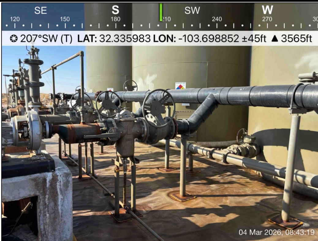
PHOTO 4: Southwestern view during liner inspection activities. 3/4/2026
