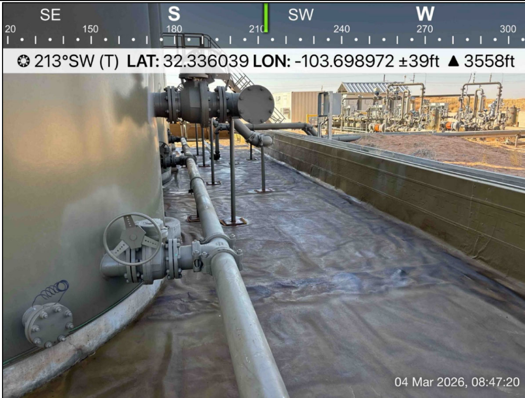
PHOTO 7: Southwestern view during liner inspection activities. 3/4/2026
