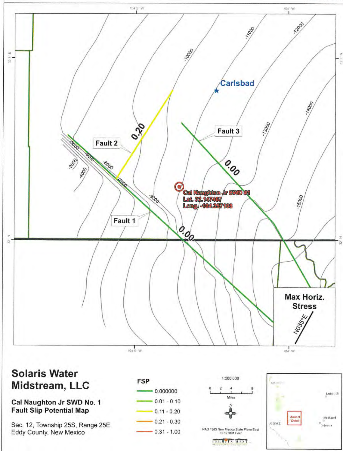
Figure 2. Detail Precambrian fault map of Cal Naughton Jr SWD #1 area as mapped by Ewing (1990). Faults are colored based on probability of fault slip as modeled using Fault Slip Potential software (Walsh and Zoback, 2016). Labeled values represent the calculated fault slip potential using the parameters indicated in Table 1. Contours show the top of the Precambrian basement in feet below sea level.
