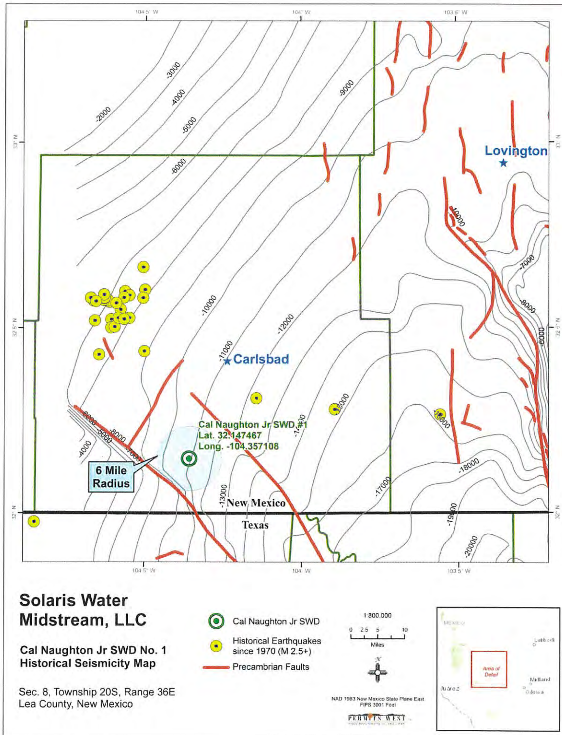
Figure 1. Structural contour map of the Precambrian basement in feet below sea level. Red lines represent the locations of Precambrian basement-penetrating faults (Ewing et al., 1990). The Cal Naughton Jr SWD #1 well lies ~6.0 miles east of the closest deeply penetrating fault and 17 miles from the closest historic earthquake.
