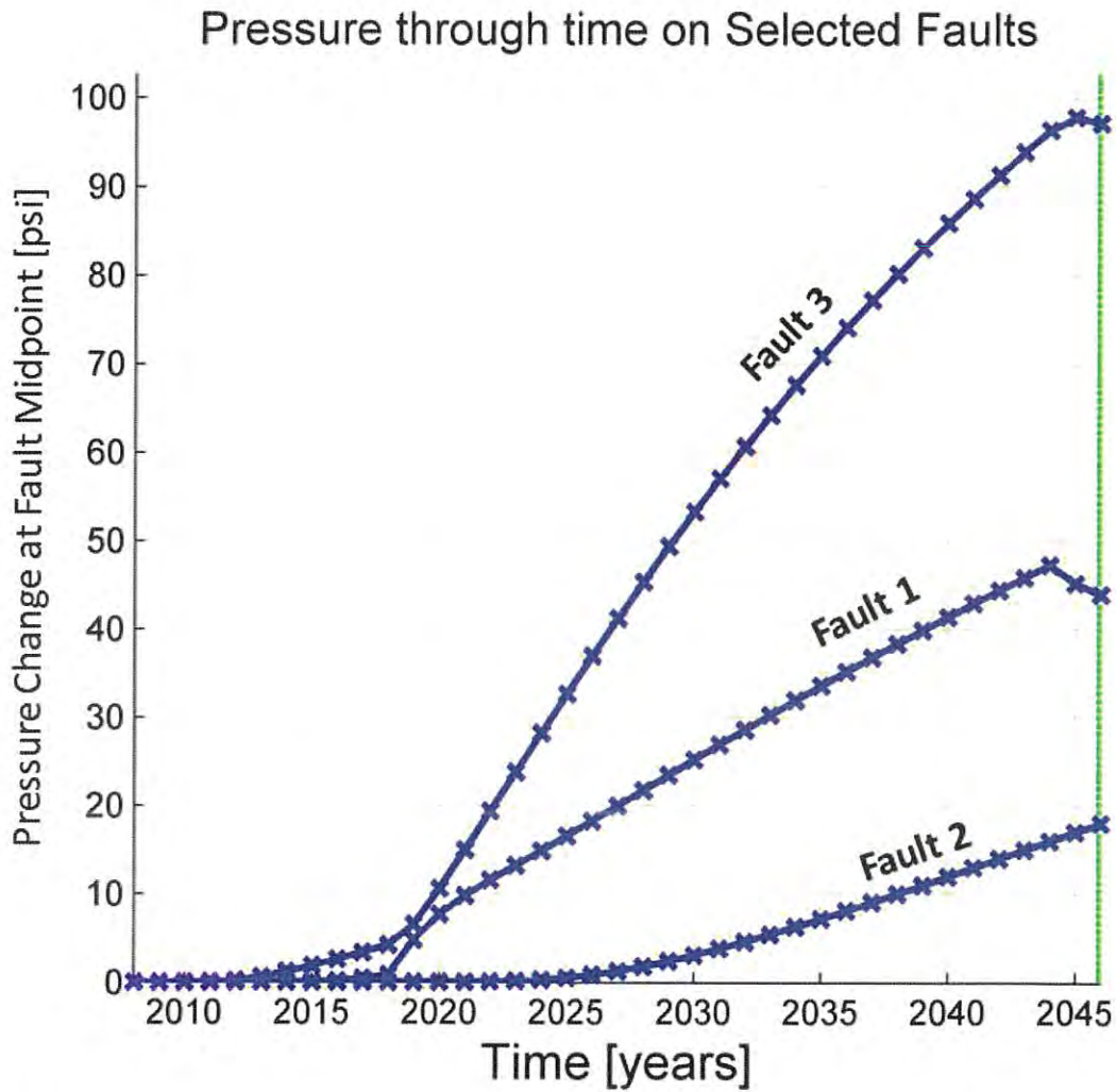
Figure 3. A scatter plot showing the modeled change of pore pressure on faults 1, 2 & 3 through time, as a response to the addition of the proposed SWD well.
