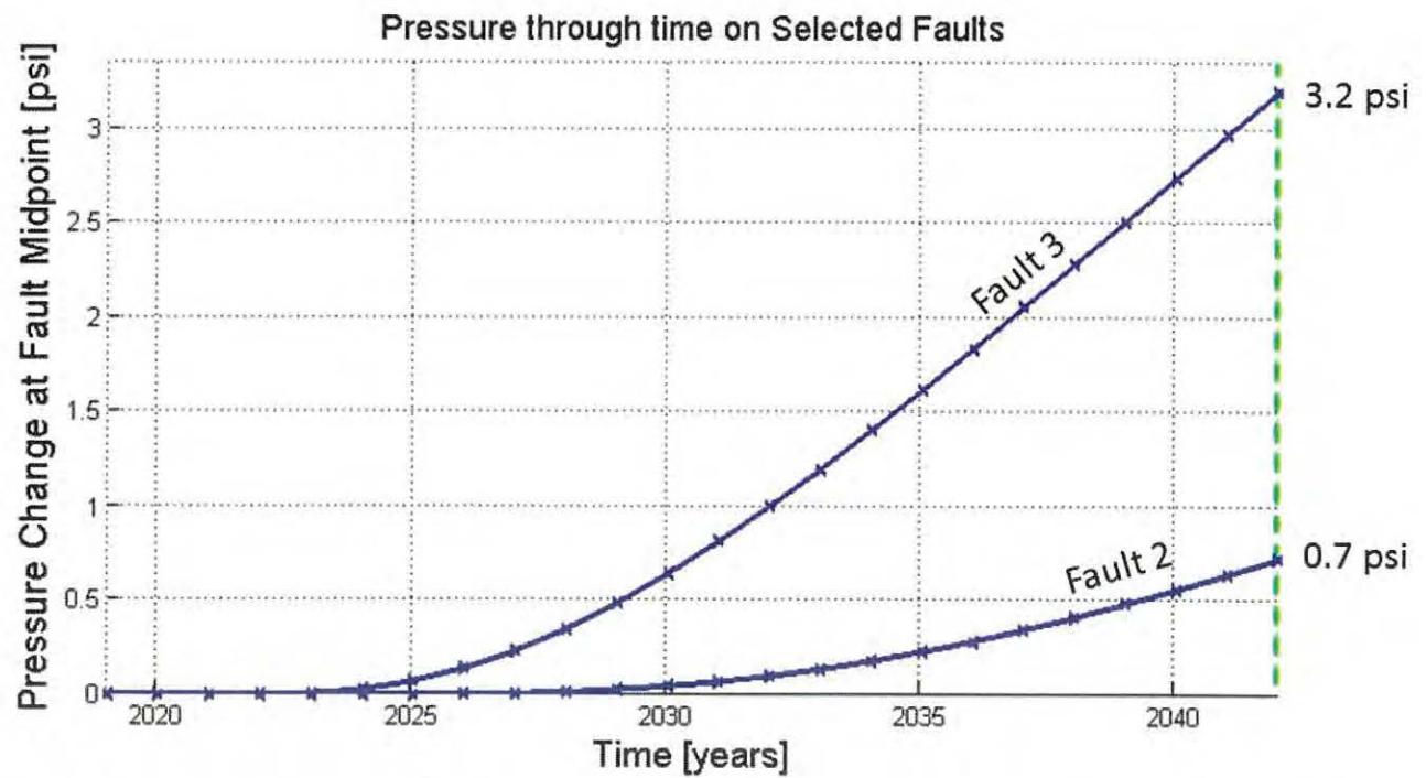
Figure 3. Scatter plots showing the modeled change of pore pressure on faults 2 and 3 through time as a response to the proposed SWD well.
