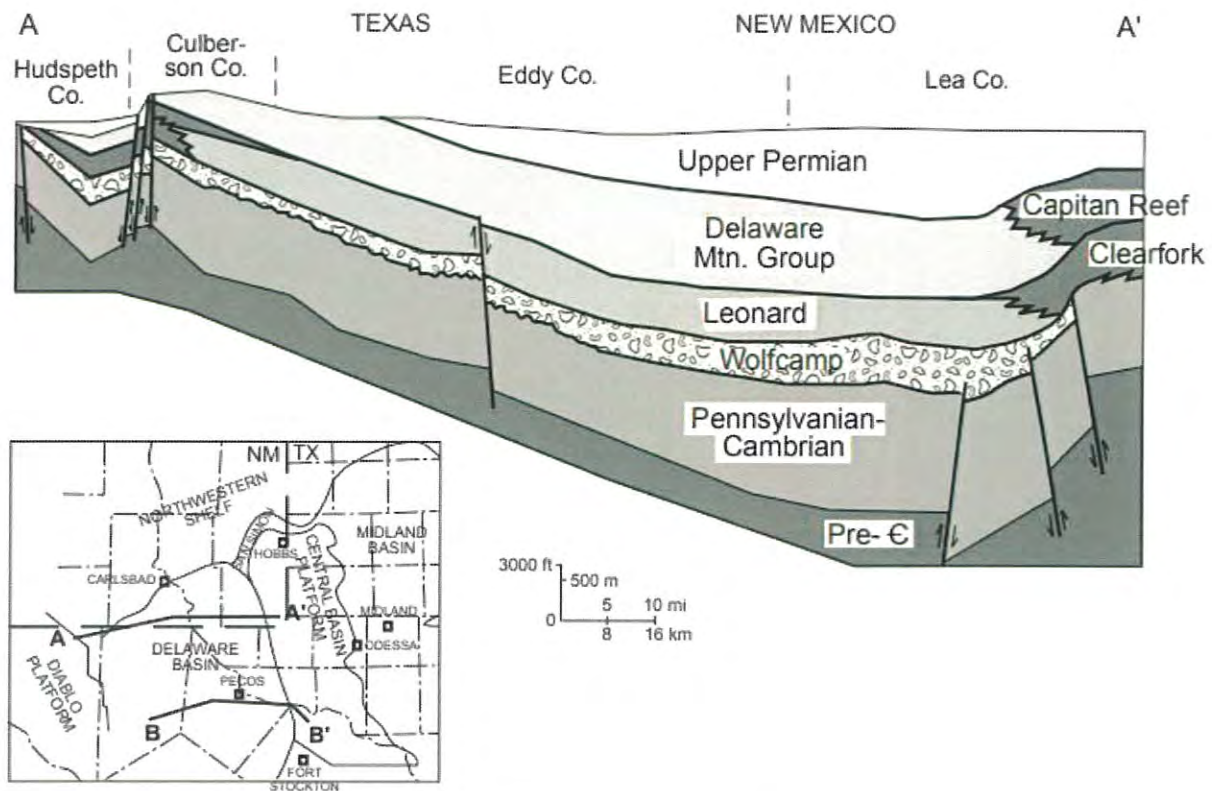
Figure 3. Cross section of the Permian Basin from Montgomery (1997). Notice the basement faults only penetrating through the Leonardian and deeper formations and not through the proposed injection zone within the Delaware Mtn. Group.
