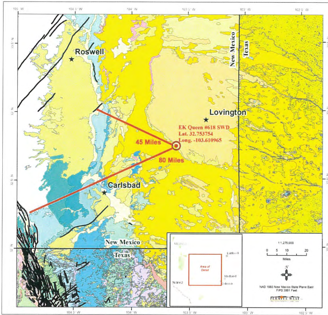
Figure 1. Geologic map of the northwestern Permian Basin. Thick black lines represent locations of fault traces and show that the nearest faults to the proposed E-K Queen Unit 618 well lie >45 miles away.
