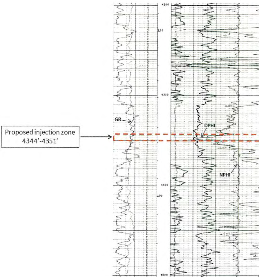
Figure 4. Well log taken from the E-K Queen Unit 618 well illustrating the proposed injection zone in a dashed red line. The injection zone is characterized by an extremely high porosity bed. The injection zone is confined on either side by a 100 ft minimum of low porosity beds of limestone, dolomite, anhydrite, etc.
