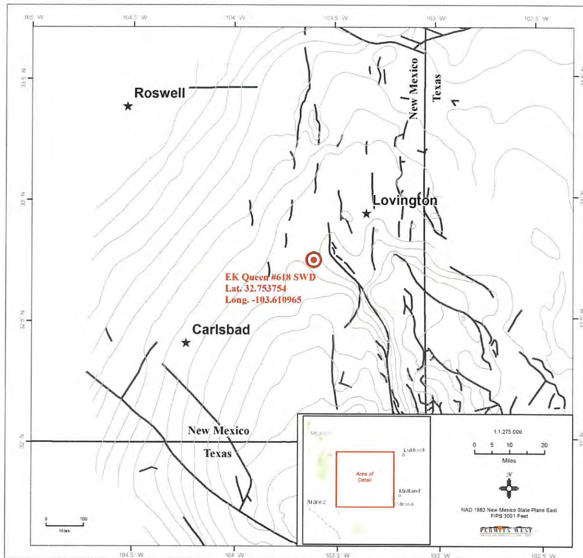
Figure 2. Structural contour map of the Paleozoic Ellenburger formation. Thick black lines represent the locations of deep Precambrian basement faults. Precambrian faults are close to the proposed well location (~5 mi), however, these faults are too deep to allow the injected fluids to travel toward the surface or cause any other concern.
