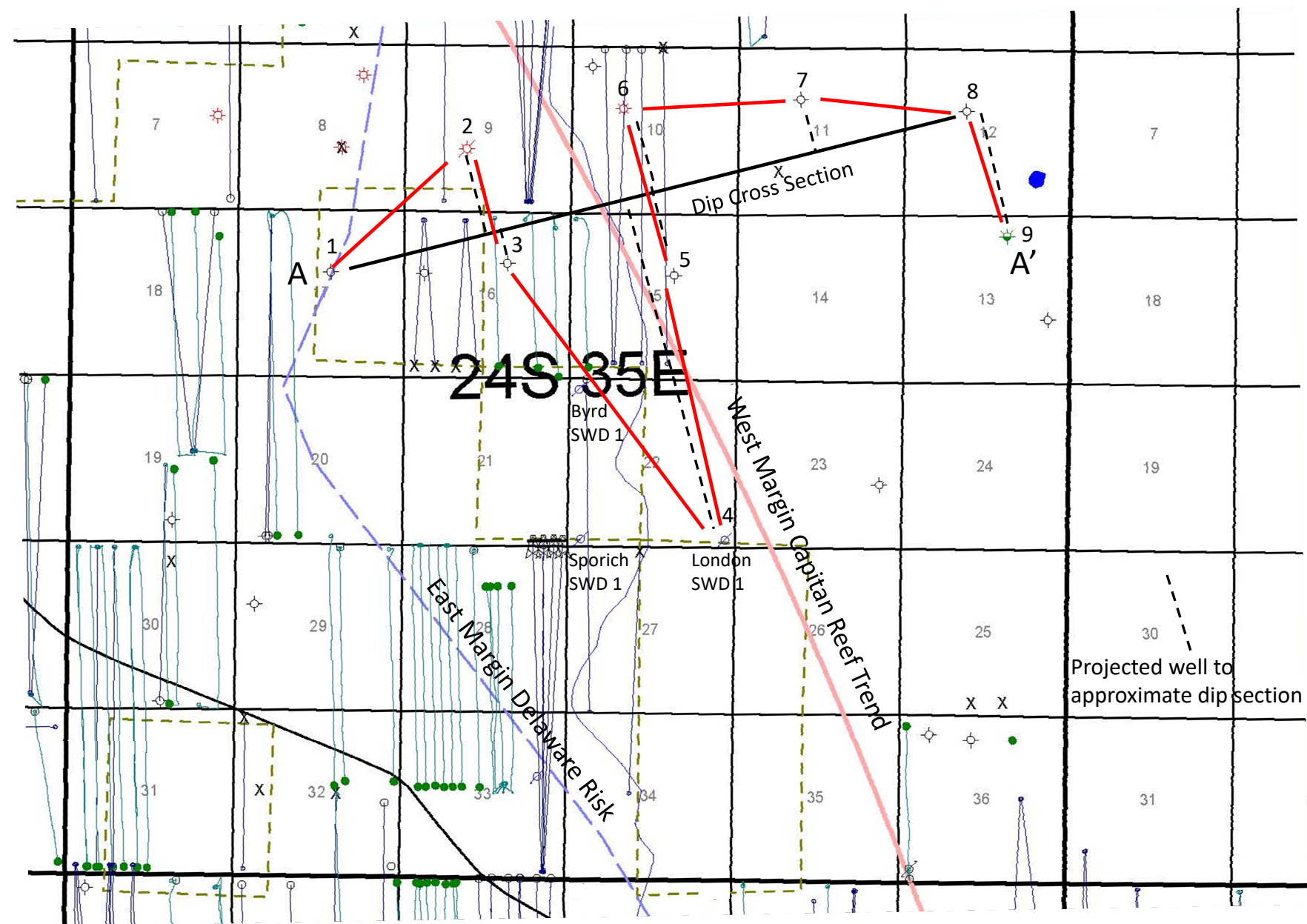
London SWD 1 Index Map Cross Section A – A'
