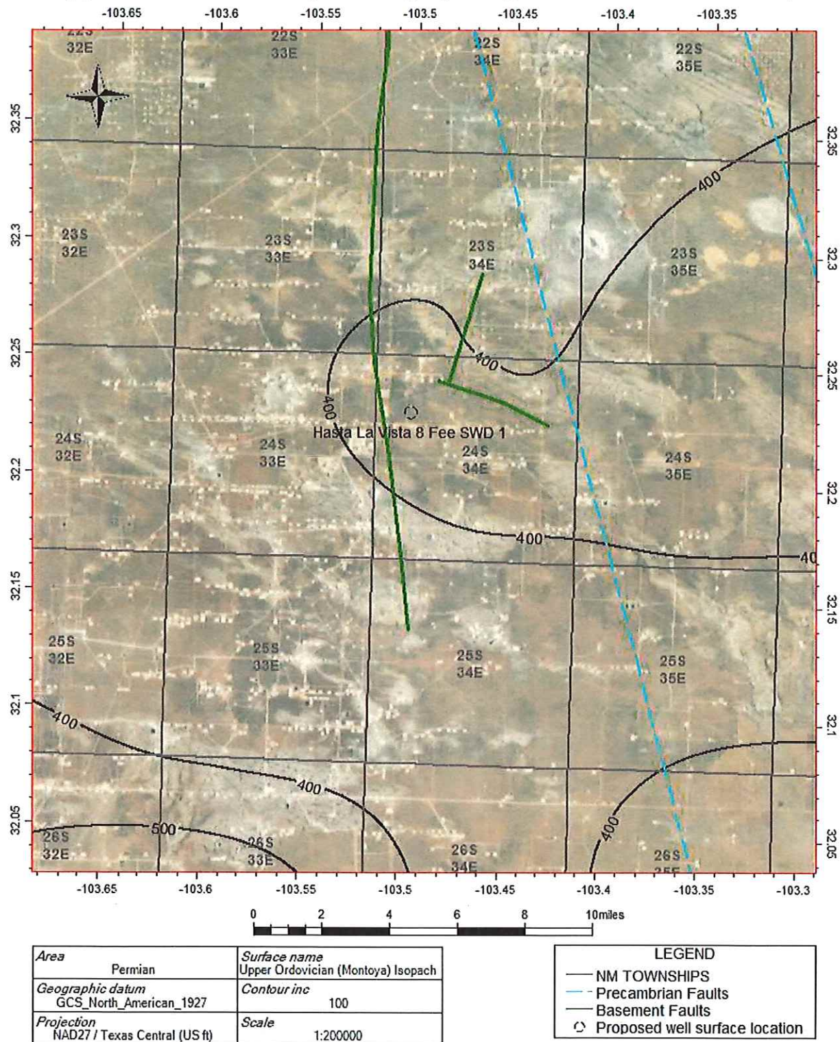
Figure 2: Upper Ordovician (Montoya) Isopach and Faults Map
