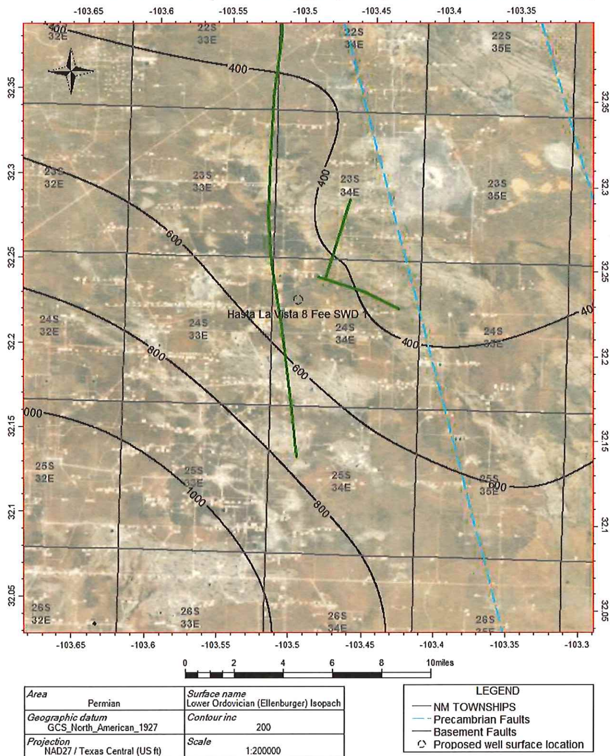
Figure 5: Lower Ordovician (Ellenburger) Isopach and Faults Map
