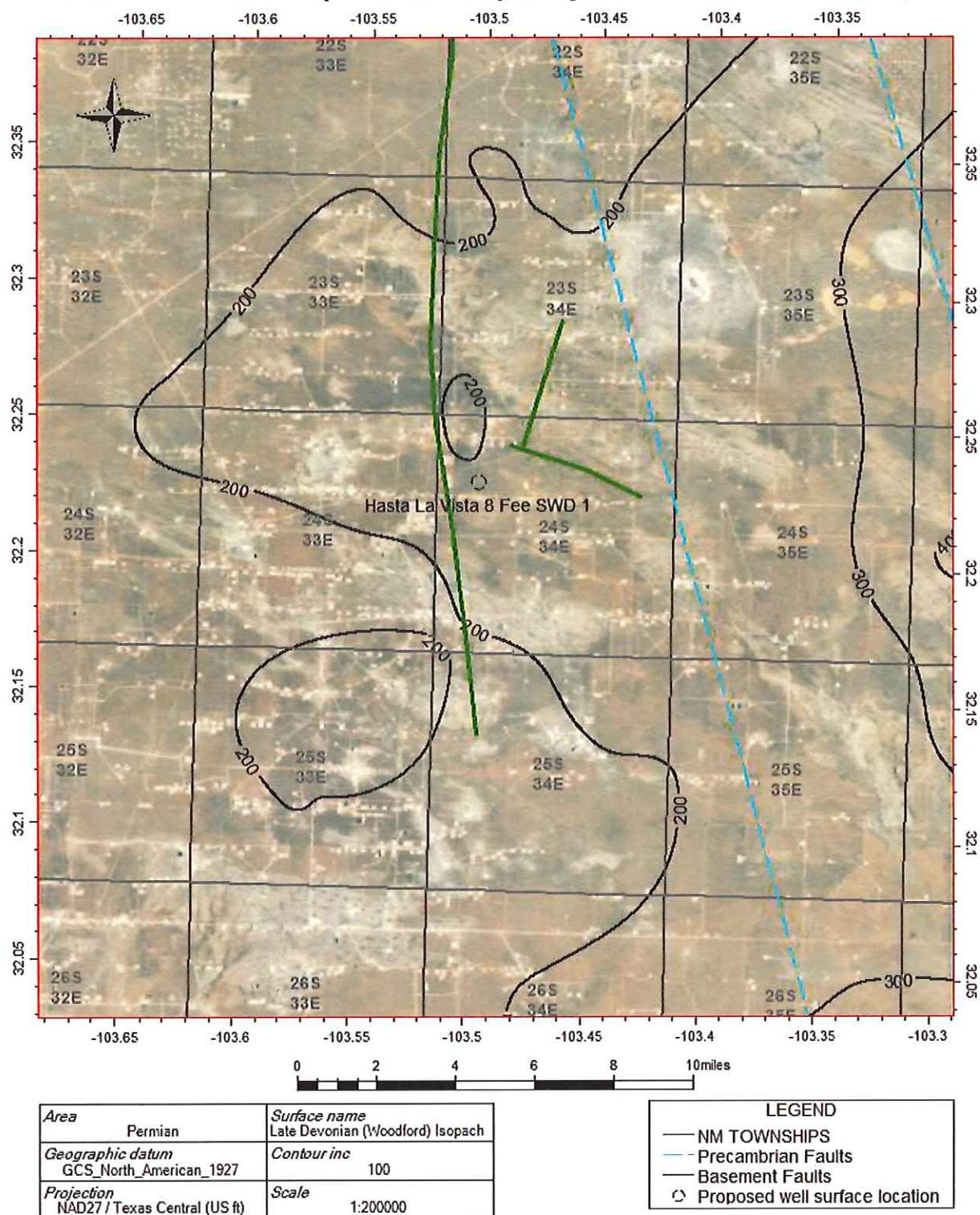
Figure 3: Late Devonian (Woodford) Isopach and Faults Map
