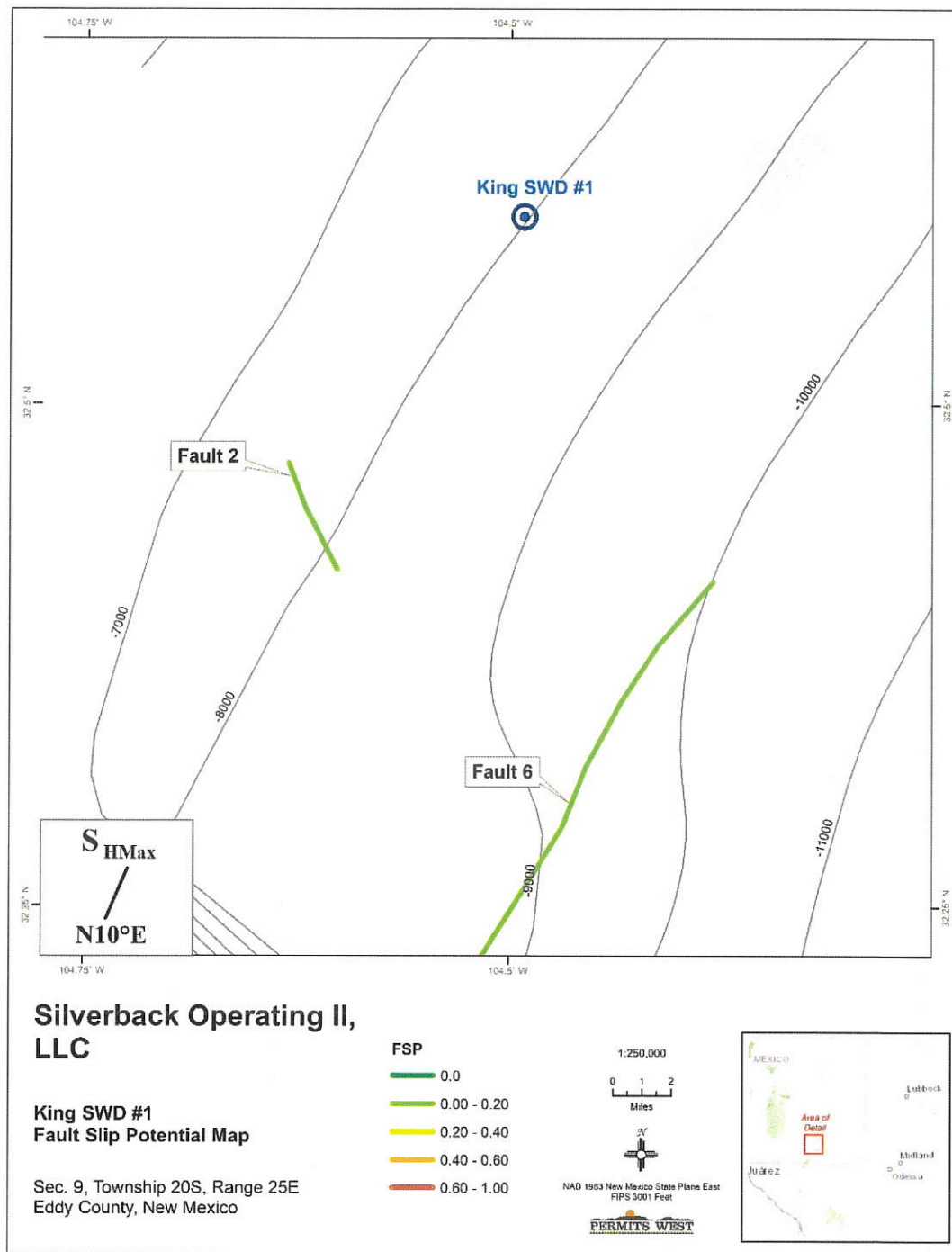
Figure 2. Precambrian fault map of the King SWD area as mapped by Ewing et al. (1990). Faults are colored based on probability of fault slip as modeled using Fault Slip Potential software (Walsh and Zoback, 2016). Labeled values represent the calculated fault slip potential using the parameters indicated in Table 2. Contours show the top of the Precambrian basement in feet below sea level.
