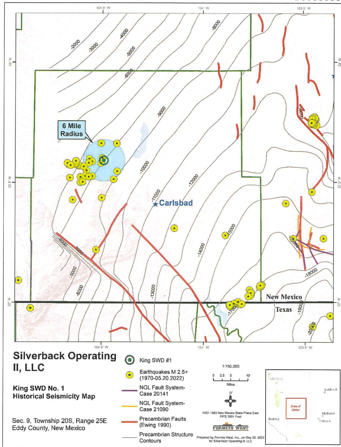
Figure 1. Structural contour map of the Precambrian basement in feet below sea level. Red lines represent the locations of Precambrian basement-penetrating faults (Ewing et al., 1990). King SWD #1 well lies ~11.7 miles northeast of the closest deeply penetrating fault and ~0.8 miles southeast from the closest historic earthquake.
