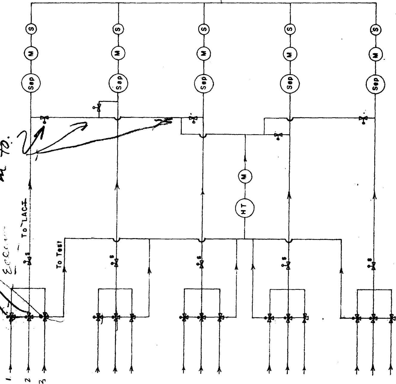
Schematic Diagram Proposed Commingling
