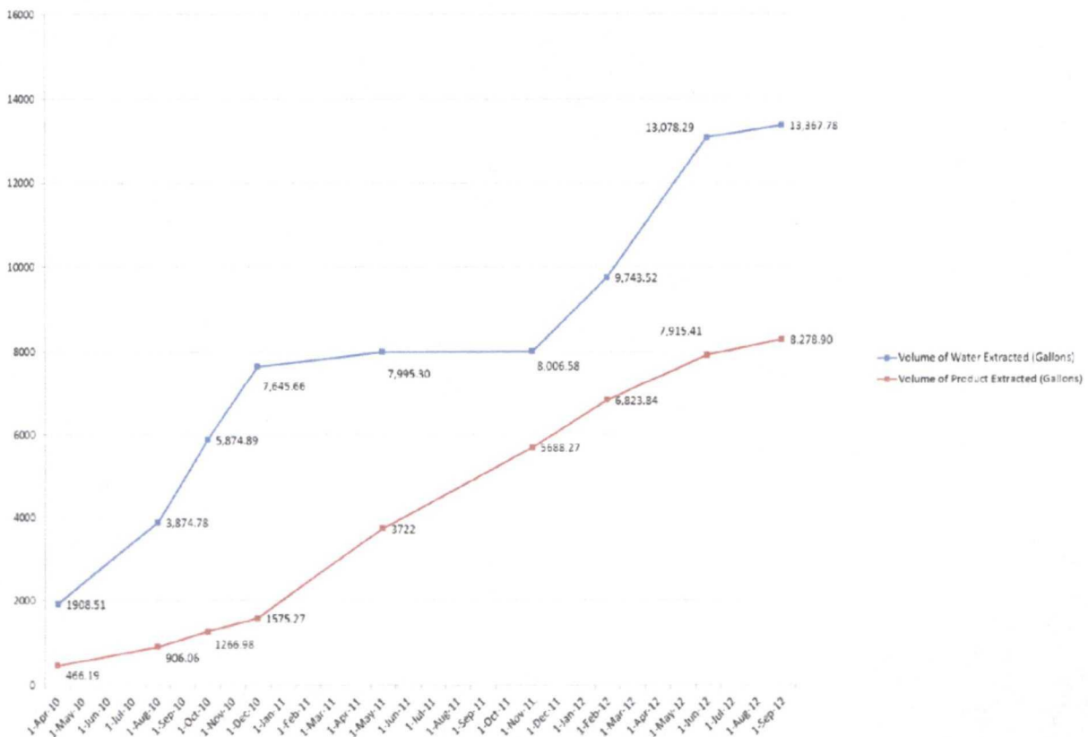
Totalized Recovered Groundwater and LNAPL Volumes Hobbs Booster Station Lea County, New Mexico
