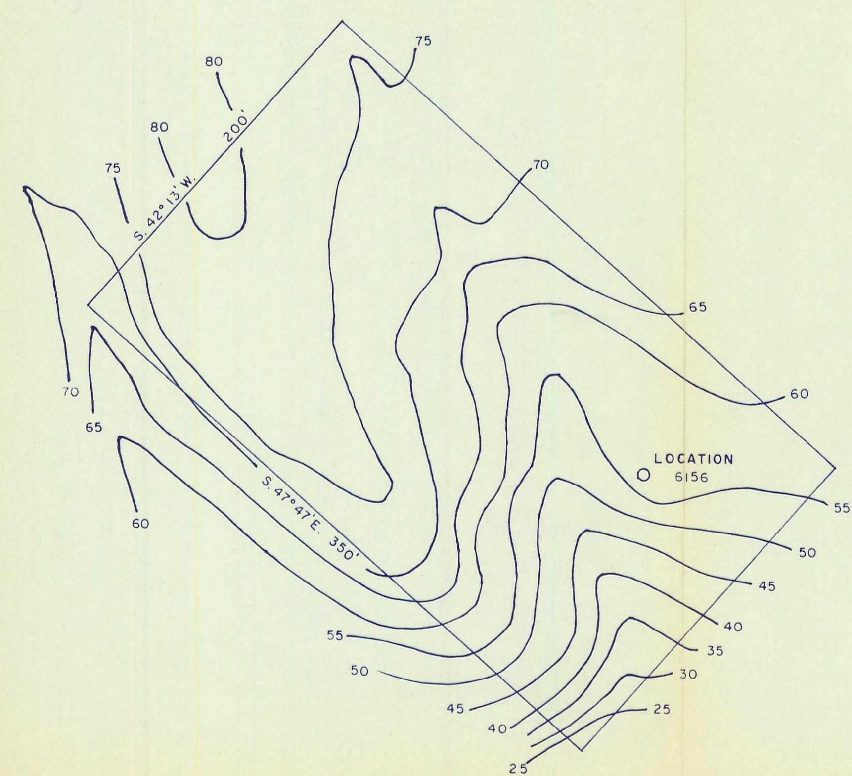
ENLARGED DIAGRAM Well Site 1" = 50'
