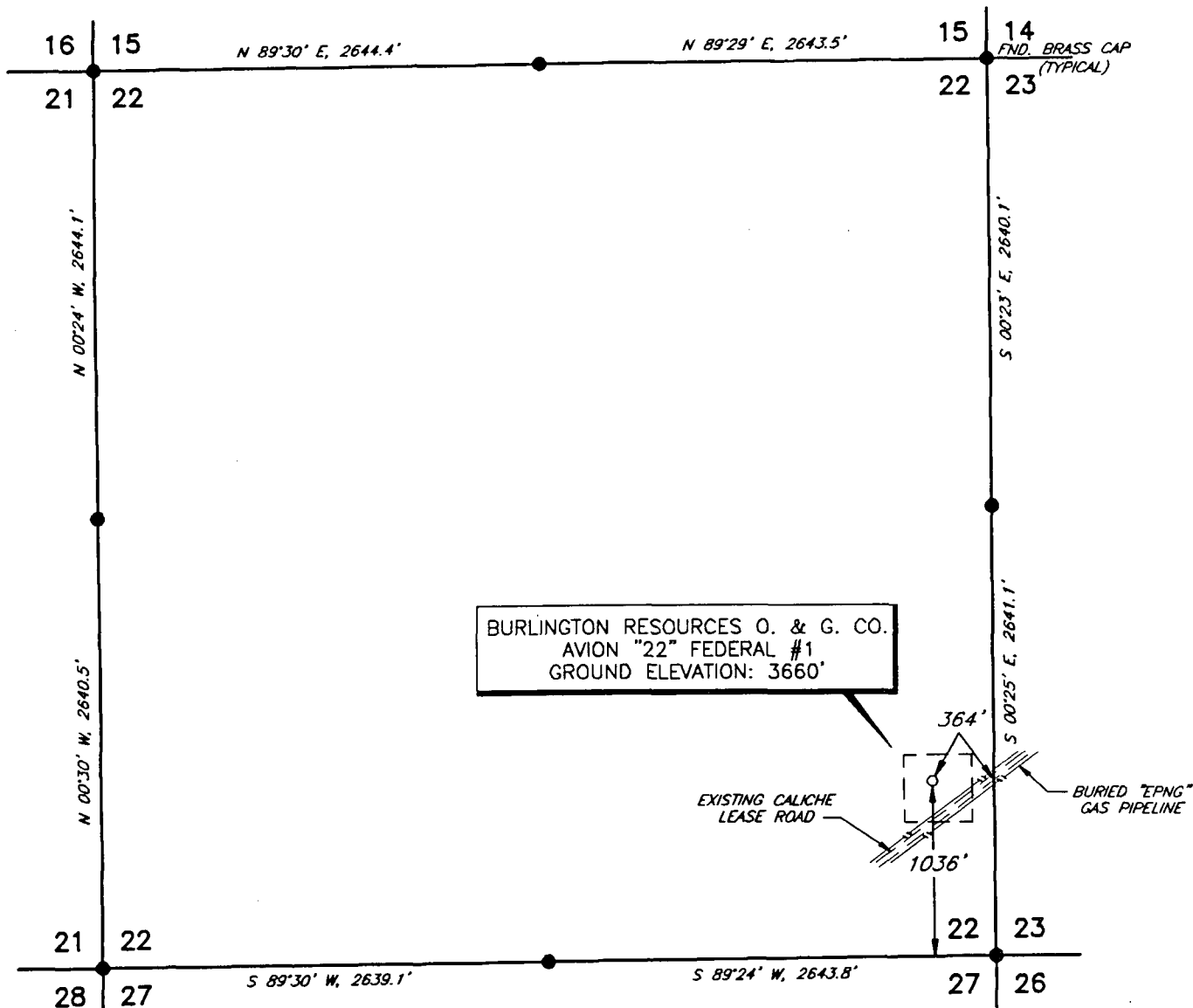
PLAN VIEW 1" = 1000'
