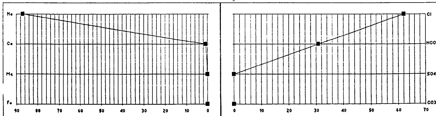
Stiff Diagram
